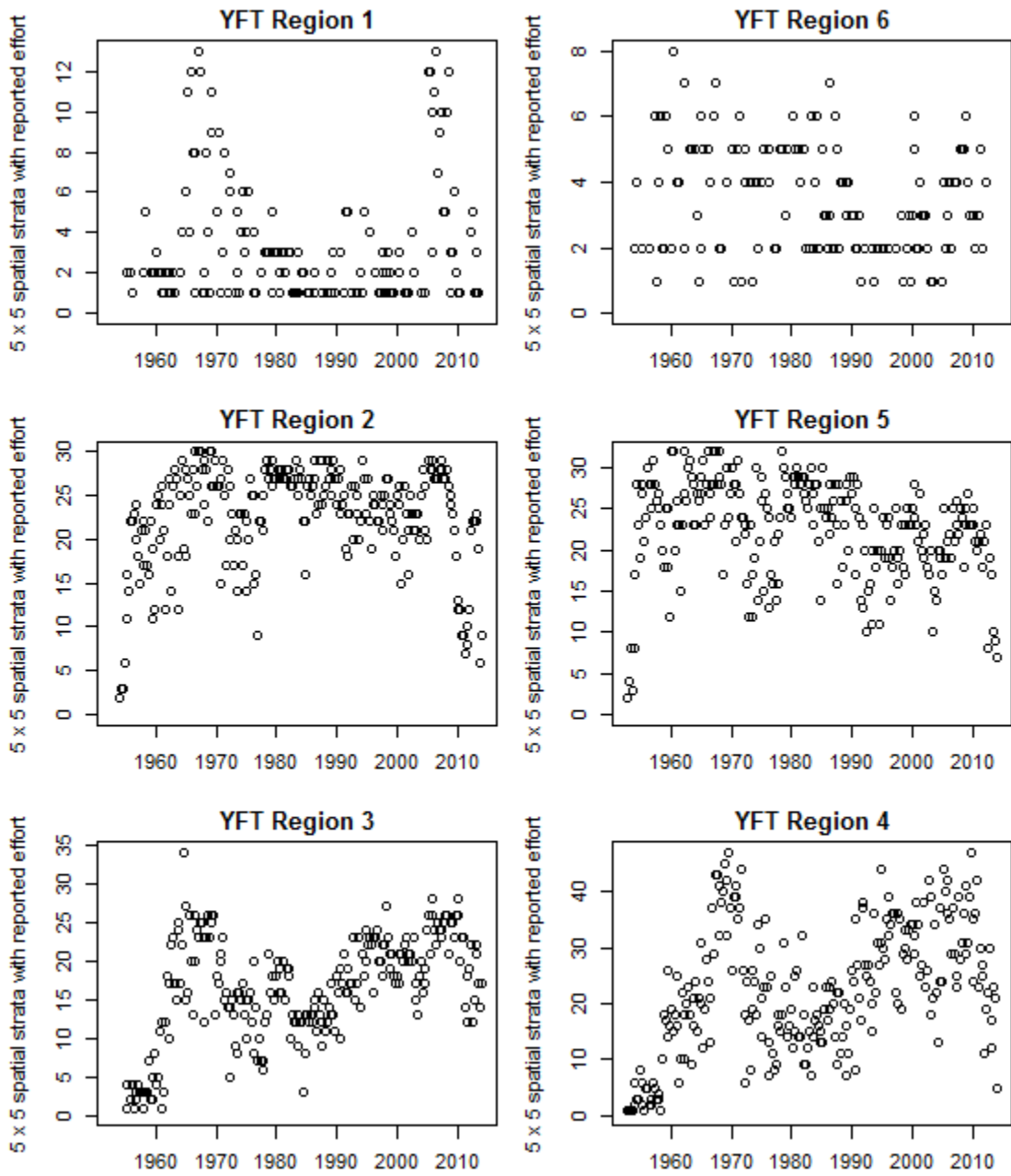
Figure 60: Number of 5 degree squares with data in the joint dataset by year-qttr and region.
