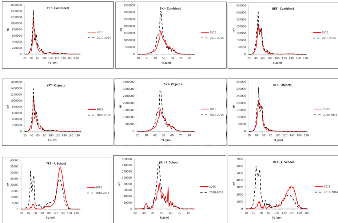
Figure 18. Size distribution of the catches by species (YFT, left; SKJ, middle; BET, right), by fishing mode (combined, top; Logs, middle; Free schools, bottom), in 2015 and on average over 2010 – 2014 period.
