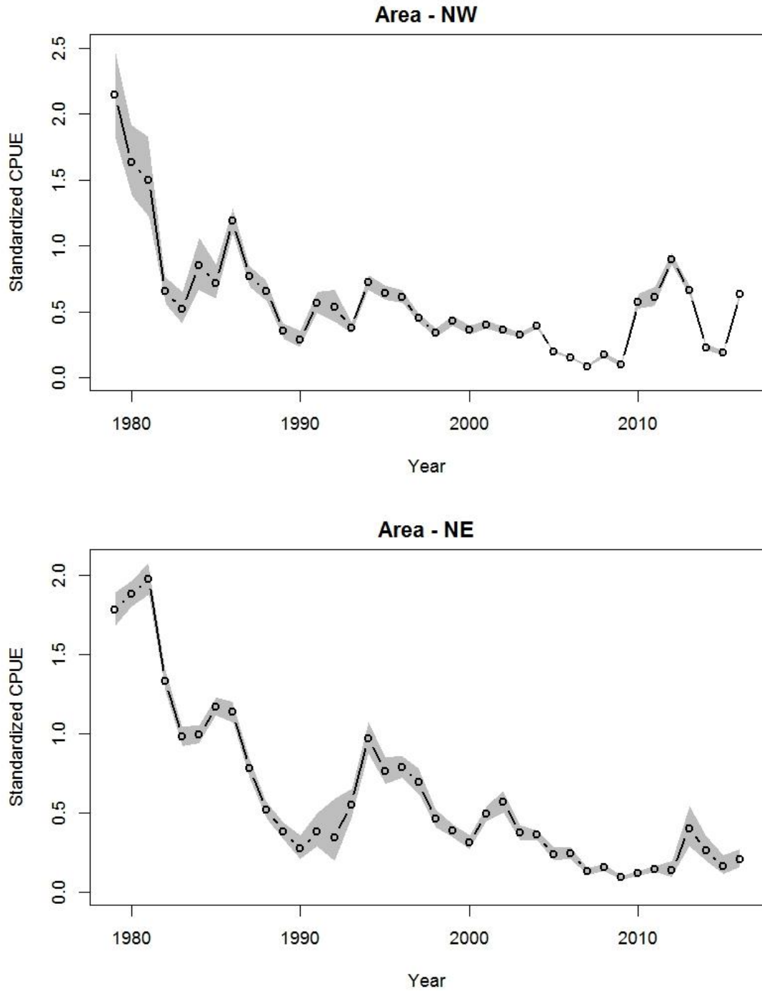
Fig. 4. Area-specific standardized (lines) CPUE with 95% confidence interval (shaded areas) for striped marlin of Taiwanese longline fishery in the Indian Ocean. CPUEs were scaled by the averaged value for each series.
