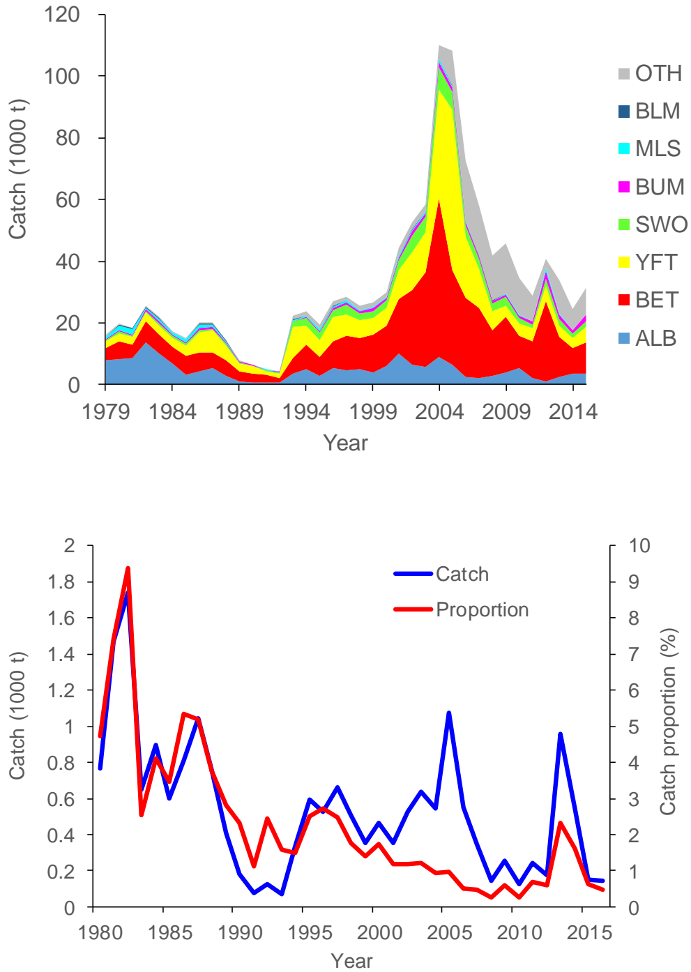
Fig. 1. Annual catches by species (upper panel) and catch of striped marlin (lower panel) caught by Taiwanese longline fishery in the Indian Ocean.
