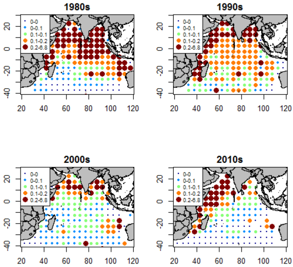
Fig. 2. Nominal CPUE distributions for striped marlin caught by Taiwanese longline fishery in the Indian Ocean.
