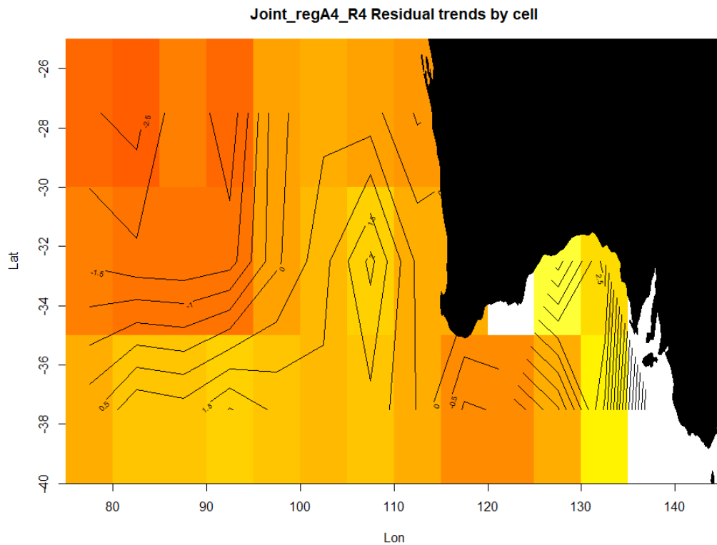
Figure 31: Trends in temporal residuals by grid cell for temperate albacore regions 3 (western, regA4_R3) and 4 (eastern, regA4_R4) from the model for 1979 to 2017 with vessel effects. The trends in each cell are estimated by regressing the residuals against year-quarter. Darker red represents decline and lighter yellow represents increase relative to the model average.
