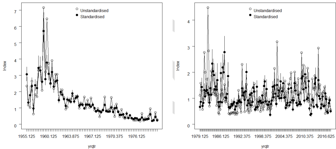
Figure 15: Comparison plot of unstandardised and standardised indices for albacore tuna in region 1 (western subtropical, regA4_R1) in the periods 1952-1979 (left) and 1979-2017 (right). NB. this plot comes from the model with HBF and not cluster.
