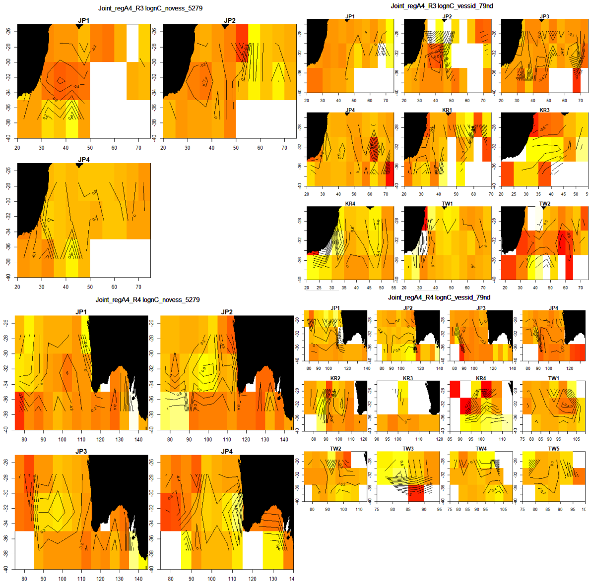
Figure 23: Albacore residuals for temperate regions 3 (regA4_R3, above) and 4 (regA4_R4, below), by cluster. Median residuals are mapped by 5° cell for the periods 1952-1979 without vessel effects (left), and 1979-2017 with vessel effects (right).
