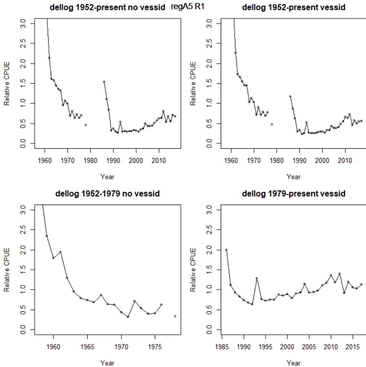
Figure 11: Annual CPUE series for albacore regional structure A5 (regA5_R1), including time series for all years (top) both with (right) and without (left) vessel effects, and time series for 1952-79 without vessel effects, and 1979-2017 with vessel effects.
