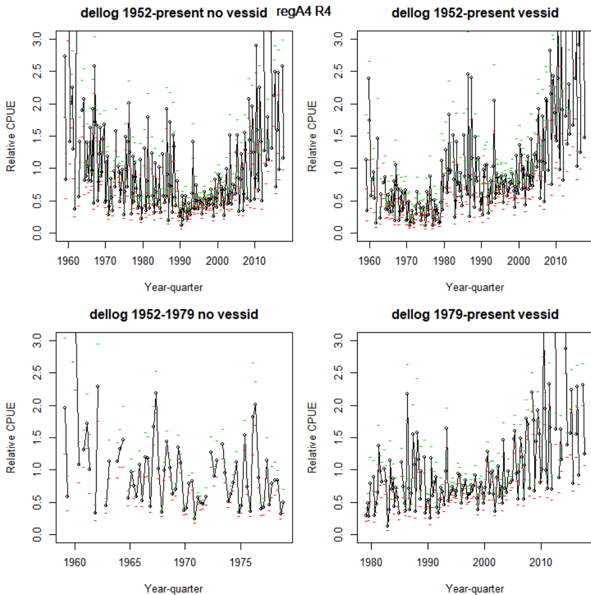
Figure 5: Quarterly CPUE series for albacore region 4 (eastern temperate, regA4_R4), including time series for all years (top) both with (right) and without (left) vessel effects, and time series for 1952-79 without vessel effects, and 1979-2017 with vessel effects.
