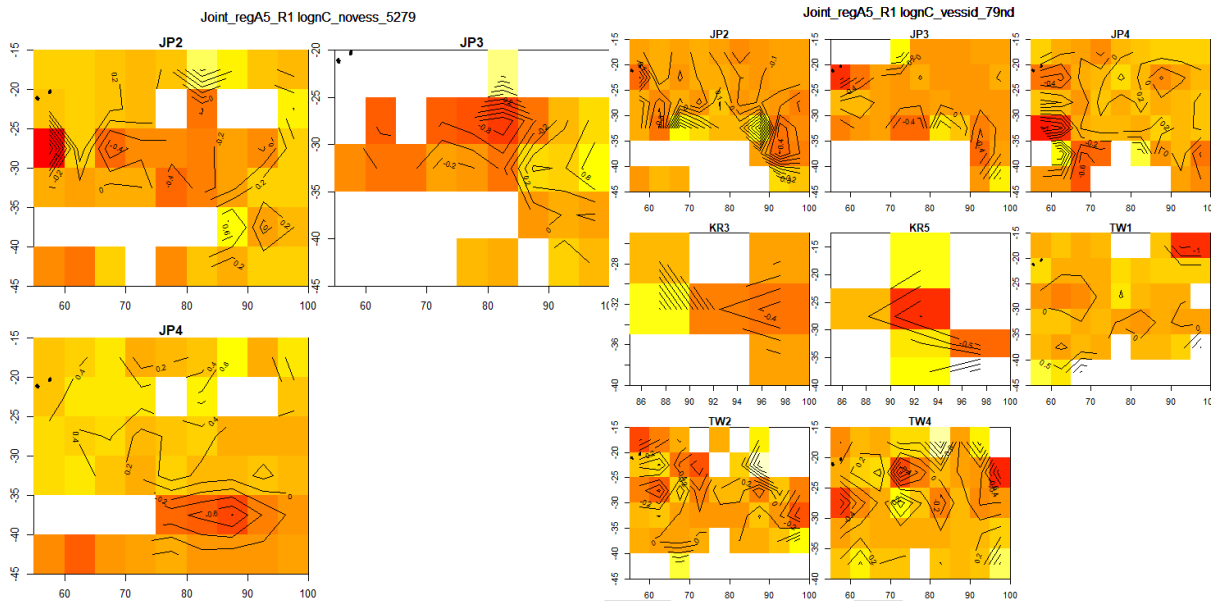
Figure 24: Albacore residuals for temperate regional structure A5 (regA5_R1) by cluster. Median residuals are mapped by 5° cell for the periods 1952-1979 without vessel effects (left), and 1979-2017 with vessel effects (right).
