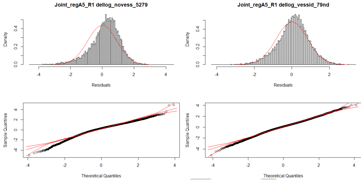
Figure 14: Diagnostic plots for albacore lognormal positive models in regional structure A5 (regA5_R1), for 1952-79 without vessel effects (left) and for 1979-2017 with vessel effects (right).
