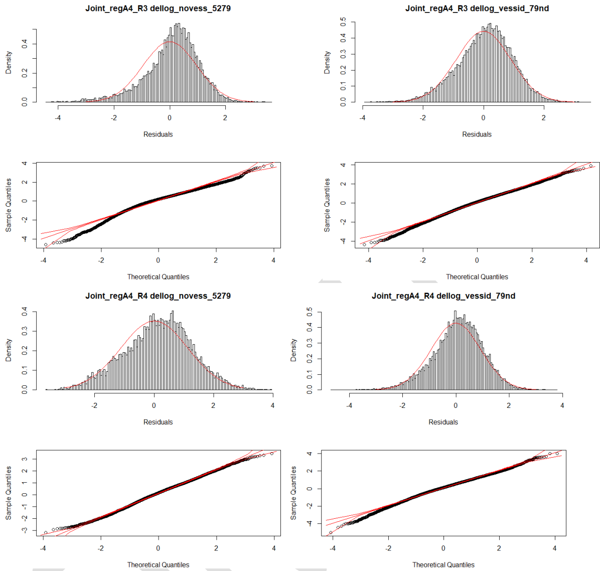
Figure 13: Diagnostic plots for albacore lognormal positive models in temperate regions 3 and 4 (regA4_R3 and regA4_R4), for 1952-79 without vessel effects (left) and for 1979-2017 with vessel effects (right).
