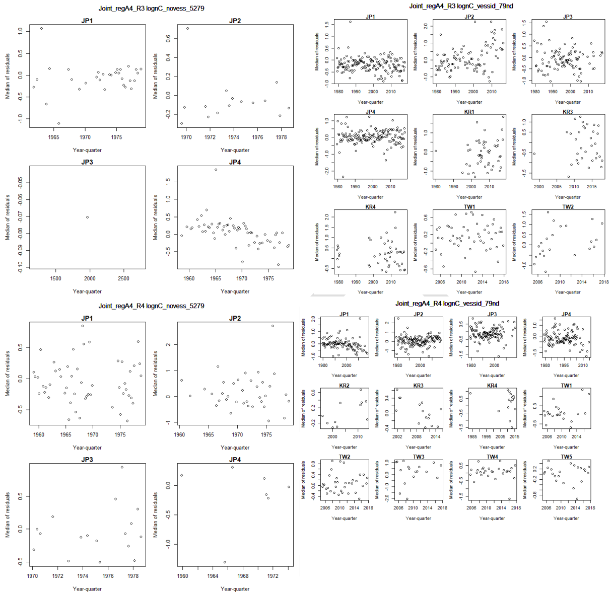
Figure 21: Median residuals from the lognormal constant model per year-quarter (x-axis), by cluster (subplots), for albacore in regions 3 (western temperate, regA4_R3, above) and 4 (eastern temperate, regA4_R4, below). Residuals are shown for 2 models: 1952-1979 without vessel effects (left), and 1979-2017 with vessel effects (right).
