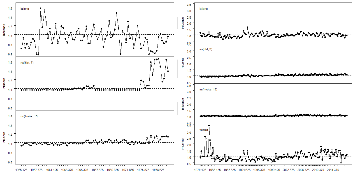
Figure 25: Influence plot for albacore region R1 (western subtropical, regA4_R1) in the periods 1952-1979 (left) and 1979-2017 (right), showing the multiplicative effect (y axis) of each variable on the standardized index. NB. This plot comes from the model with HBF and not cluster.
