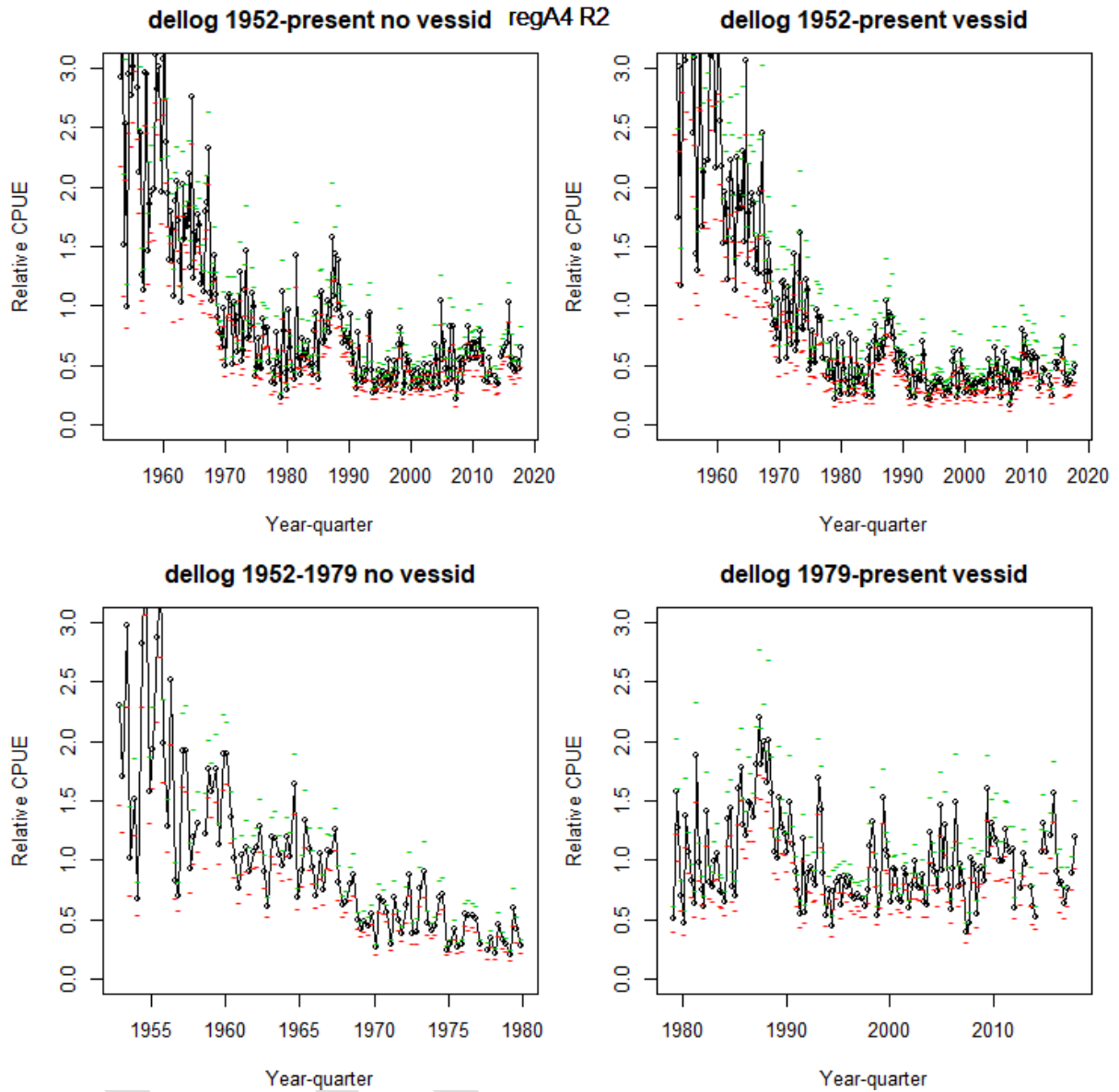
Figure 3: Quarterly CPUE series for albacore region 2 (eastern subtropical, regA4_R2) in regional structure A4. The plots include time series for all years (top) both with (right) and without (left) vessel effects, and time series for 1952-79 without vessel effects, and 1979-2017 with vessel effects.
