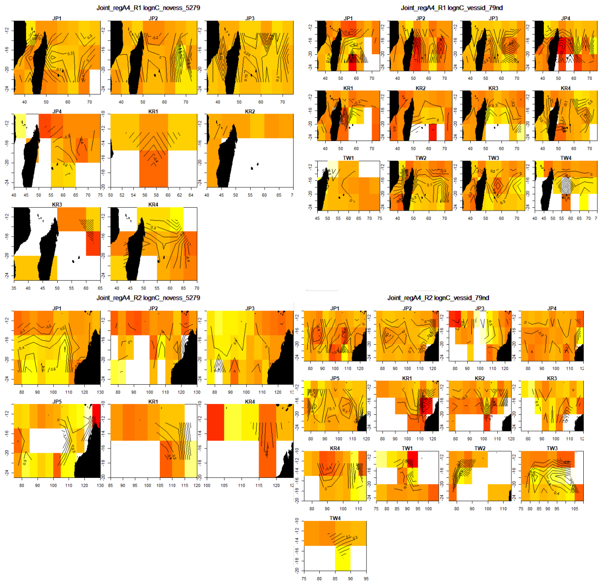
Figure 22: Albacore residuals for subtropical regions 1 (regA4_R1, above) and 2 (regA4_R2, below), by flag. Median residuals are mapped by 5° cell for the periods 1952-1979 without vessel effects (left), and 1979-2017 with vessel effects (right).
