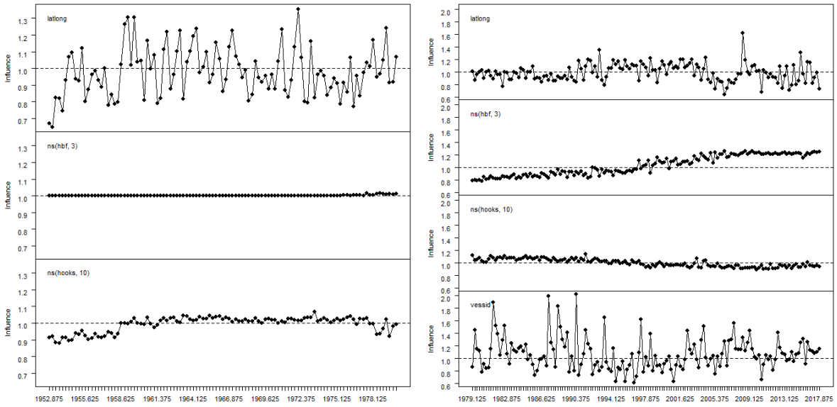
Figure 26: Influence plot for albacore region 2 (eastern subtropical, regA4_R2) in the periods 1952-1979 (left) and 1979-2017 (right), showing the multiplicative effect (y axis) of each variable on the standardized index. NB. This plot comes from the model with HBF and not cluster.
