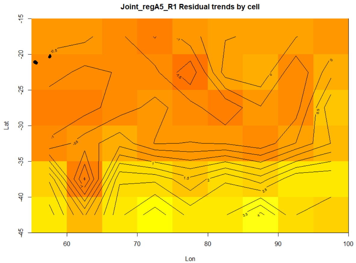
Figure 32: Trends in temporal residuals by grid cell for albacore regional structure A5 (regA5_R1) from the model for 1979 to 2017 with vessel effects. The trends in each cell are estimated by regressing the residuals against year-quarter. Darker red represents decline and lighter yellow represents increase relative to the model average.
