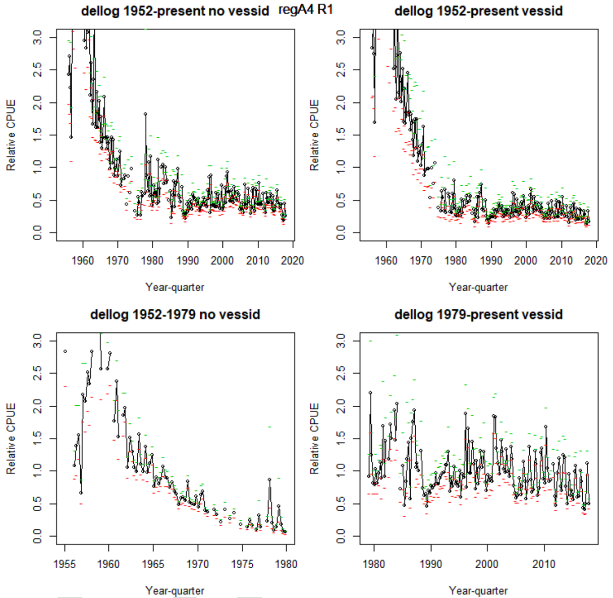
Figure 2: Quarterly CPUE series for albacore region 1 (western subtropical, regA4_R1), including time series for all years (top) both with (right) and without (left) vessel effects, and time series for 1952-79 without vessel effects, and 1979-2017 with vessel effects.
