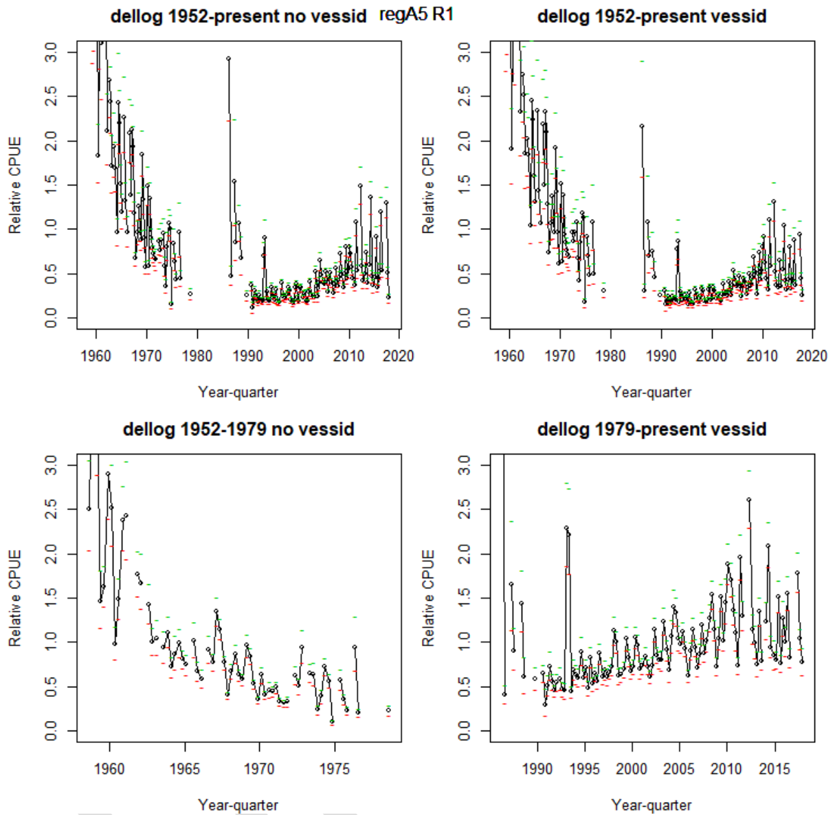
Figure 6: Quarterly CPUE series for albacore regional structure A5 (regA5_R1), including time series for all years (top) both with (right) and without (left) vessel effects, and time series for 1952-79 without vessel effects, and 1979-2017 with vessel effects.
