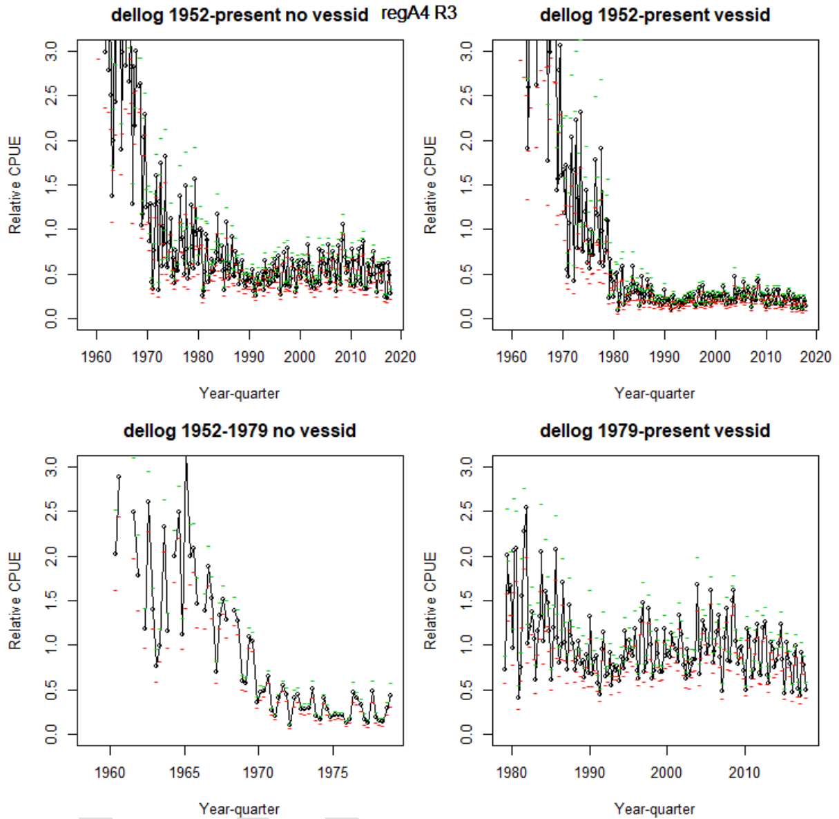
Figure 4: Quarterly CPUE series for albacore region 3 (western temperate, regA4_R3), including time series for all years (top) both with (right) and without (left) vessel effects, and time series for 1952-79 without vessel effects, and 1979-2017 with vessel effects.
