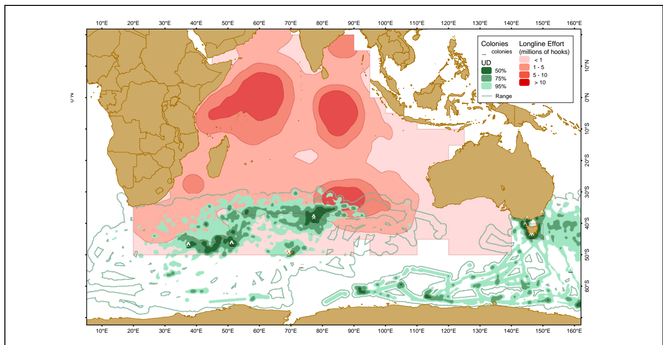
Fig. 1. Distribution of breeding albatrosses, petrels and shearwaters in the Indian Ocean (see Table 2 for a list of species included), and overlap with IOTC longline fishing effort for all gear types and fleets (average annual number of hooks set per 5° grid square from 2002 to 2005).
