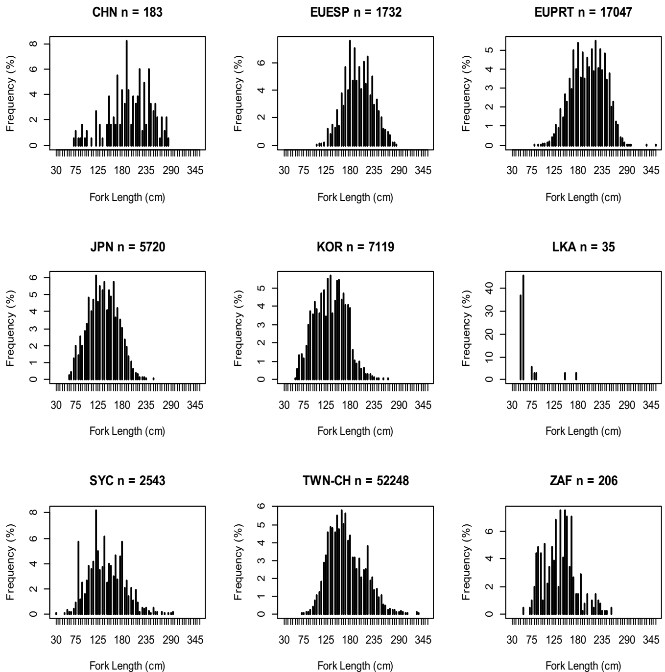
Fig. 4. Fork length frequency distributions (%) of blue shark derived from the samples reported for the longline fleets of China (CHN LL), EU, Spain (EUESP ELL), EU, Portugal (EUPRT ELL), Japan (JPN LL), Korea (KOR LL), Sri Lanka LKA (G/L), Seychelles (SYC LL), Taiwan, China (TWN FLL/LL) and South Africa (ZAF ELL) between 2005 and 2015 in 5 cm length classes.
