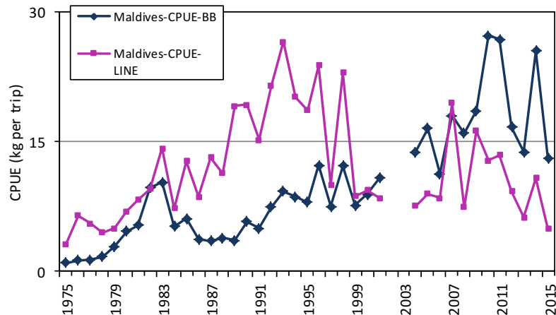
Fig. 4. Kawakawa: Nominal CPUE series for the baitboat (BB) and troll line (TROL) fisheries of Maldives (1975–2015) derived from the available catches and effort data.
