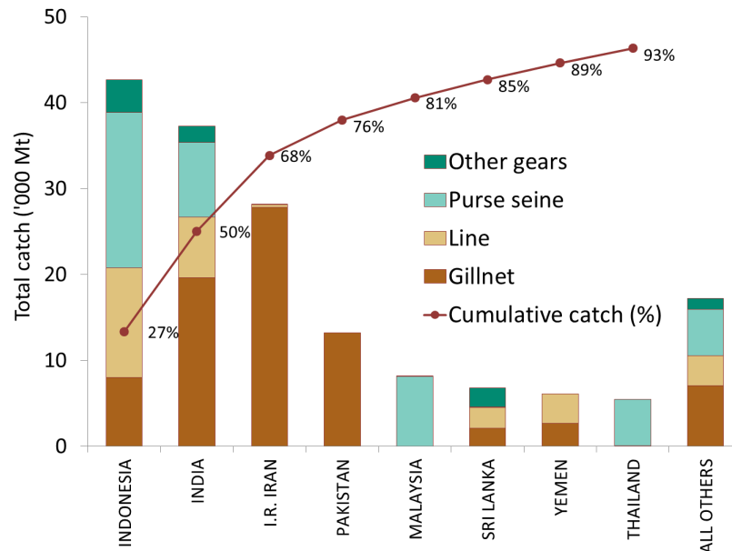
Fig. 2. Kawakawa: Average catches in the Indian Ocean over the period 2012–15, by country. Countries are ordered from left to right, according to the importance of catches of kawakawa reported. The red line indicates the (cumulative) proportion of catches of kawakawa for the countries concerned, over the total combined catches of this species reported from all countries and fisheries (data as of October 2016).
