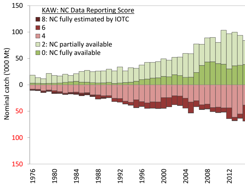
Fig. 3. Kawakawa: nominal catch; uncertainty of annual catch estimates (1976–2015). Catches are assessed against IOTC reporting standards, where a score of 0 indicates catches that are fully reported according to IOTC standards; catches assigned a score of between 2 – 6 do not report catch data fully by gear and/or species (i.e., partially adjusted by gear and species by the IOTC Secretariat) or any of the other reasons provided in the document; catches with a score of 8 refer to fleets that do not report catch data to the IOTC (estimated by the IOTC Secretariat) (data as of October 2016).
