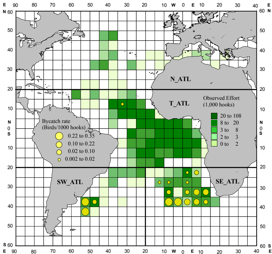
Figure 4 Observed effort distribution and average nominal incidental catch rate (birds/1000 hooks) of Taiwanese pelagic longline fleets in 5*5-degree grid from 2004 to 2008.
