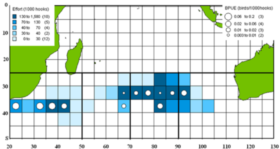
Figure 7 Effort and incidental catch per unit effort of seabirds and Distribution of SBT fleet in the Indian Ocean between 2003 and 2012
