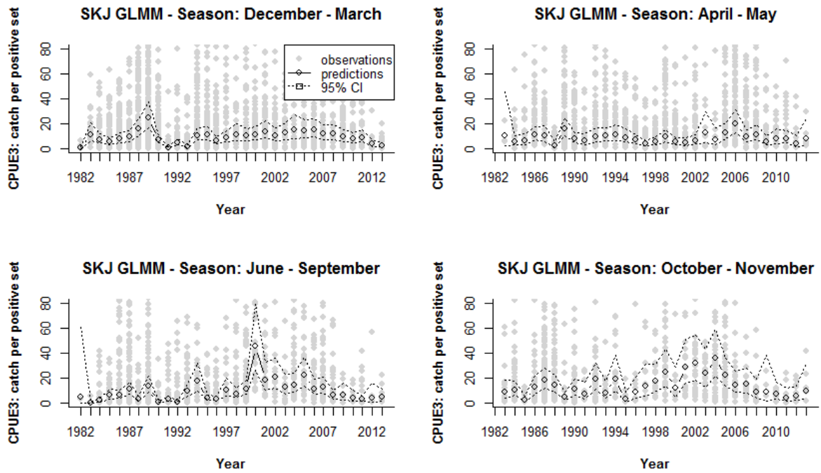
Fig 6. Catch per positive set (CPUE3) trends for skipjack, standardised using a GLMM that accounts for spatial heterogeneity of fishing effort and makes predictions for "unfished" areas.
