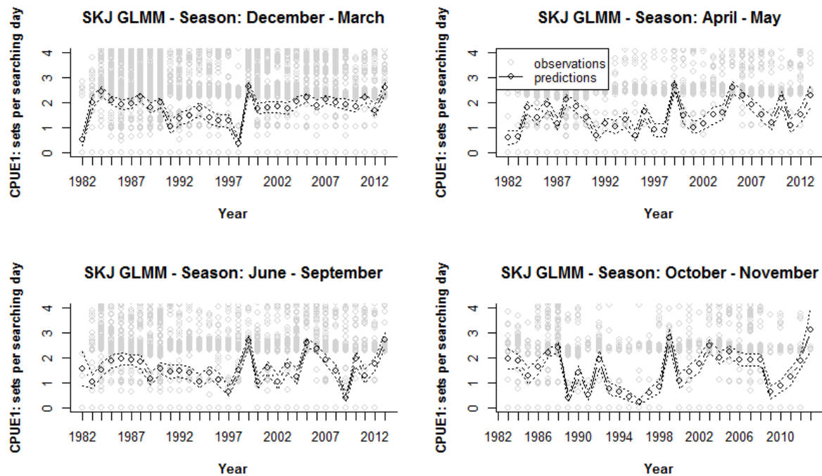
Fig 4. Sets per searching day (CPUE1) trends for skipjack, standardised using a GLMM that accounts for spatial heterogeneity of fishing effort and makes predictions for "unfished" areas.
