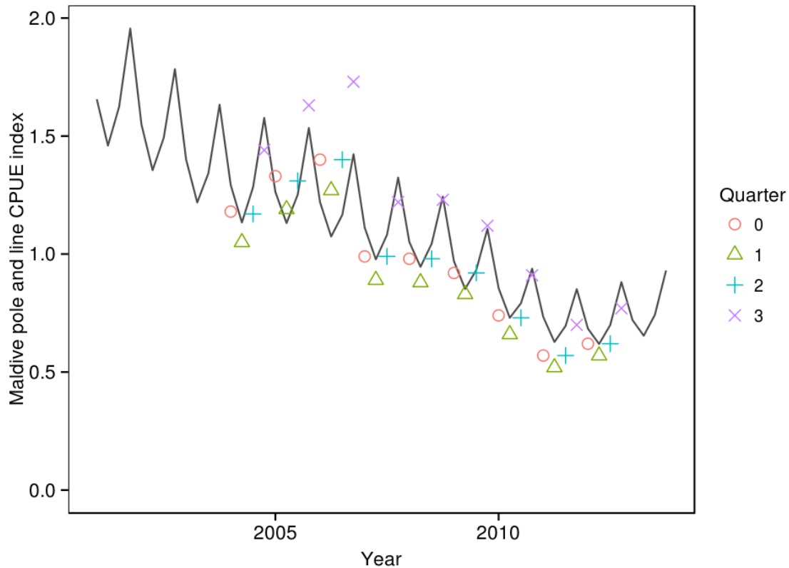
Figure 1 : Observed (points) and expected (lines) Maldivé (M) pole and line (PL) CPUE.
