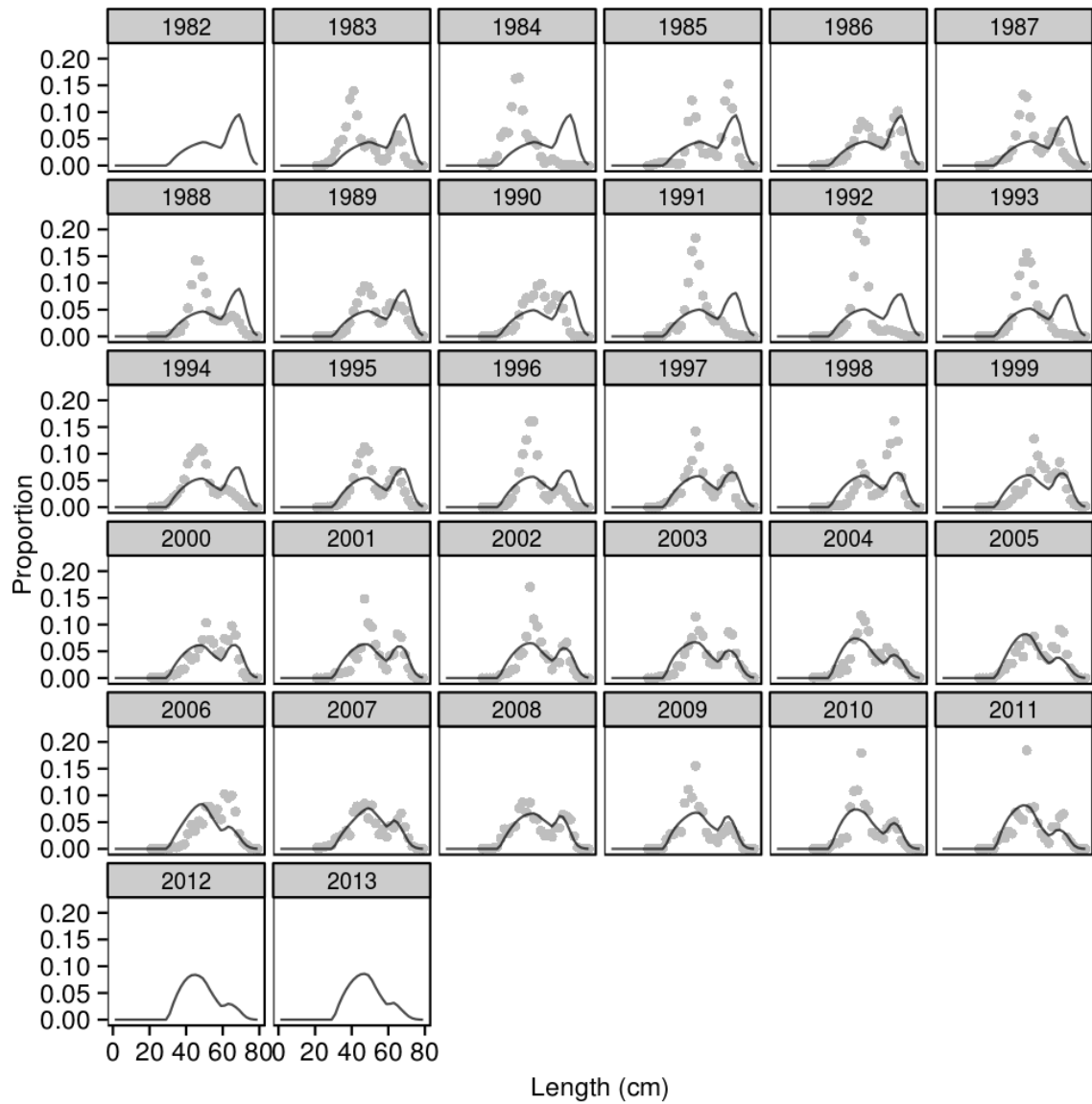
Figure 8 : Observed (points) and expected (lines) size frequency distributions for pole and line (PL) in the Maldives region (M)
