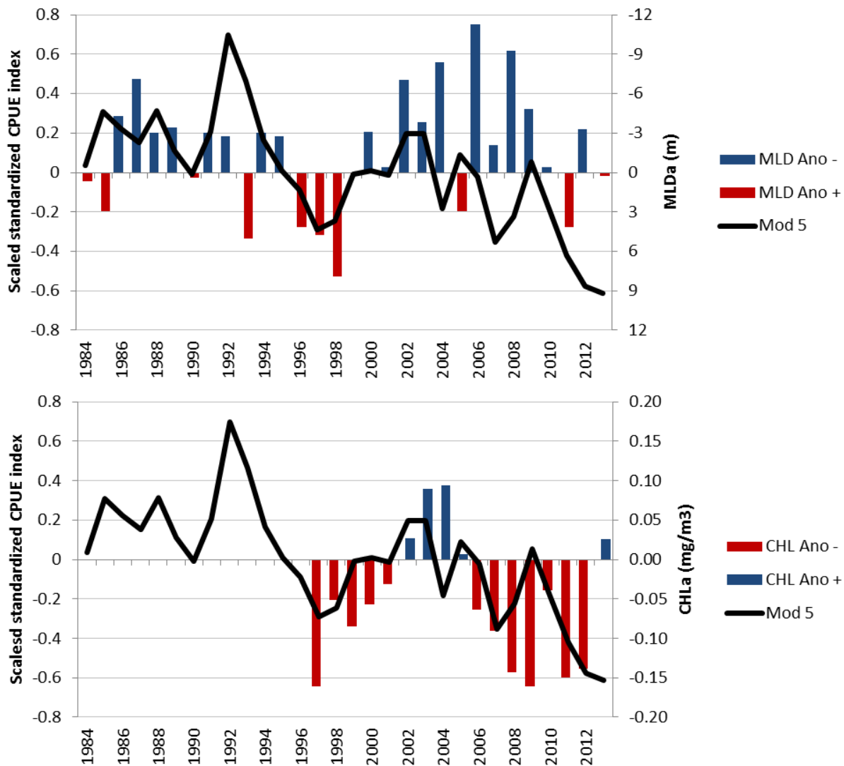
Fig. 10 – Combined series of Model 5 (NEQ, July-November) standardized CPUE? mixed layer depth anomalies (top) and chlorophyll anomalies (bottom) in the Somali basin. A negative MLDa reflects a shoaling of the thermocline, a positive MLDa indicates a deepening of the thermocline
