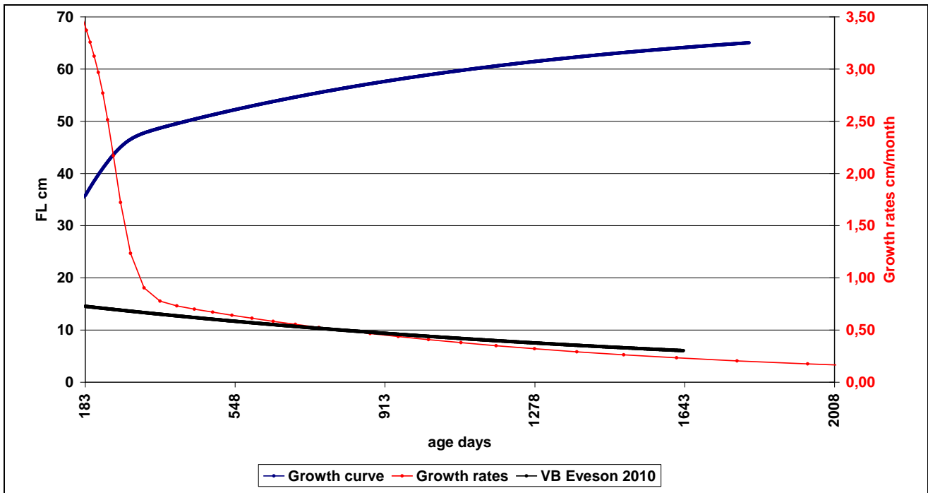
Figure 3: Growth curve and growth rates at size proposed for the Indian Ocean skipjack by Eveson et al 2014 (and growth rates at age previously estimated by Eveson et al using a VB model)
