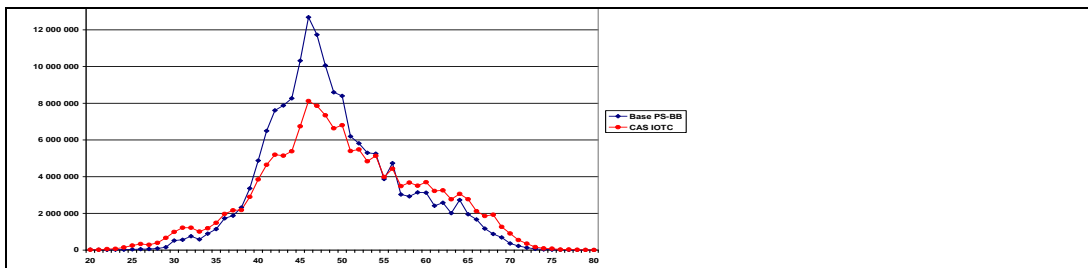
Figure 2: Comparison of the 2 skipjack CAS vectors used in the present work
