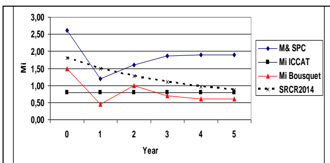
Figure 7: Yearly approximate levels of the various natural mortality at age estimated for skipjack
