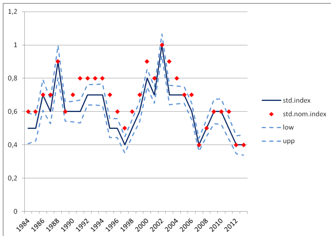
Figure 2: Standardized relative EU Purse Seine CPUE for skipjack in the Indian Ocean. Confidence intervals and nominal values are also plotted.
