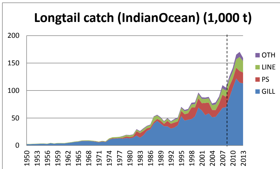
Fig. 1 Nominal longtail catch (1950-2013) by gear type (IOTC database) (April, 2015) (Note) Others include longline, bait boat and all other gear types. The broken vertical line shows 2008.
