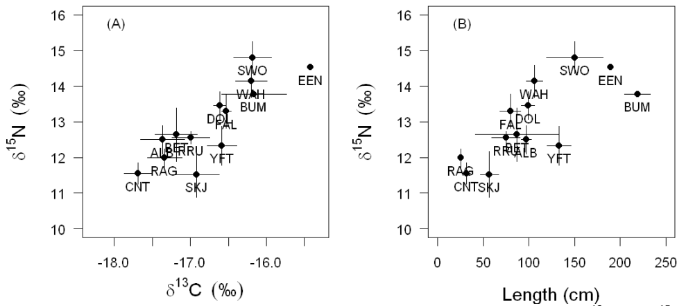
Fig. 1. Plots of mean±standard deviation of (A) carbon and nitrogen stable isotope ratios ( \delta^{13}\text{C} and \delta^{15}\text{N} ), and (B) fish size and \delta^{15}\text{N} for oceanic pelagic fish species caught in the western-central Indian Ocean. ALB = Albacore tuna, BET = Bigeye tuna, BUM = Blue marlin, CNT = Rough triggerfish, DOL = Dolphinfish, EEN = Giant grouper, FAL = Silky shark, RAG = Indian mackerel, RRU = Rainbow runner, SKJ = Skipjack tuna, SWO = Swordfish, WAH = Wahoo, YFT = Yellowfin tuna.
