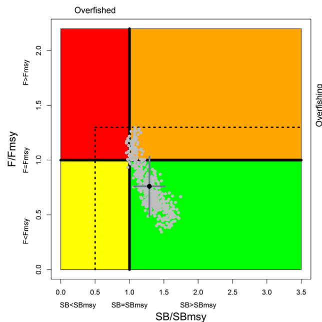
Figure. 1. Bigeye tuna: SS3 Aggregated Indian Ocean assessment Kobe plot. Dotted black lines are the interim limit reference points adopted by the Commission via Resolution 15/10. The grey points represent 500 estimates of 2015 stock status from the six model options. The black point represents the average of the six model options with associated 80% confidence interval.
