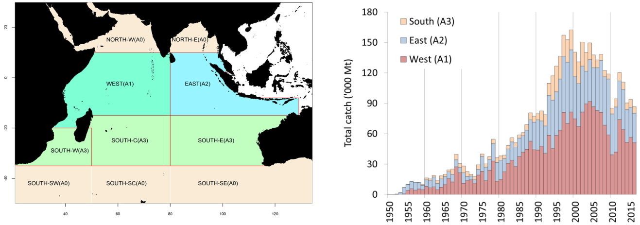
Fig. 4(a-b). Bigeye tuna: Catches of bigeye tuna by (SS3) stock assessment area by year (1950–2016). Catches outside the areas presented in the map were assigned to the closest neighbouring area for the assessment. Data as of September 2017.
