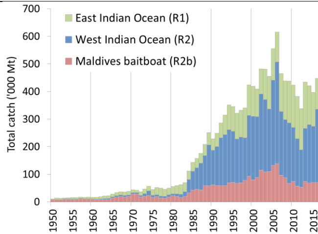
Fig. 11. Skipjack tuna: Catches of skipjack tuna by area by year estimated for the WPTT (1950–2015). Areas: East Indian Ocean (R1); West Indian Ocean (R2); Maldives baitboat (R2b). Data as of September 2017.
