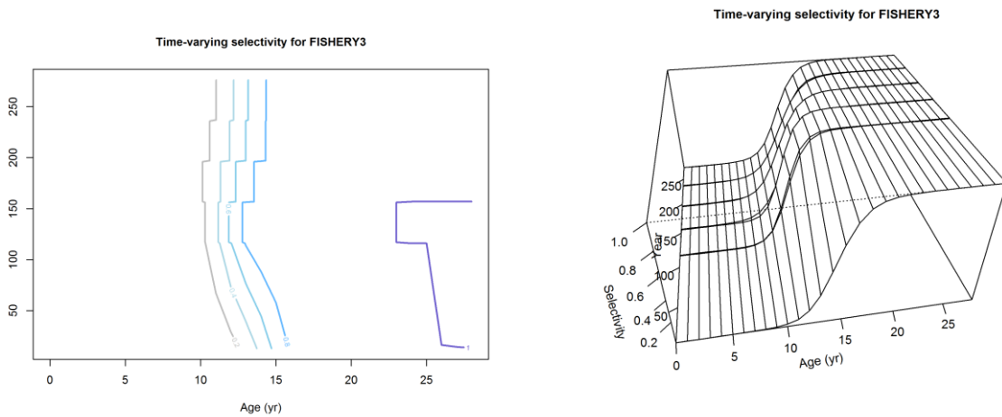
Figure 25. Longline selectivity estimated for robustness scenario NS - showing a shift toward the preference of younger ages over the first 35 years, and a shift toward older ages over the final 30 years (time axes are in quarters). Other assumptions defined as in OM-SA-analogue.
