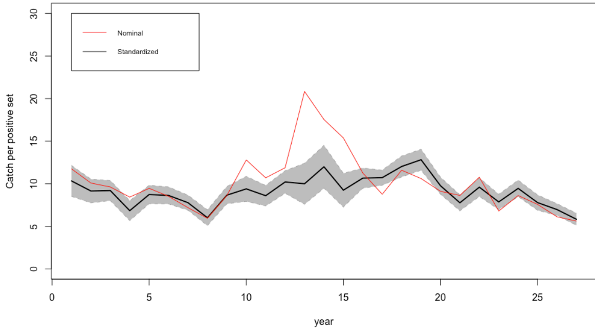
Figure 15. FSC sets – catch | catch > 0 with large YFT: standardised time series by year (black) with 97.5% confidence intervals (grey) compared to nominal (red)
