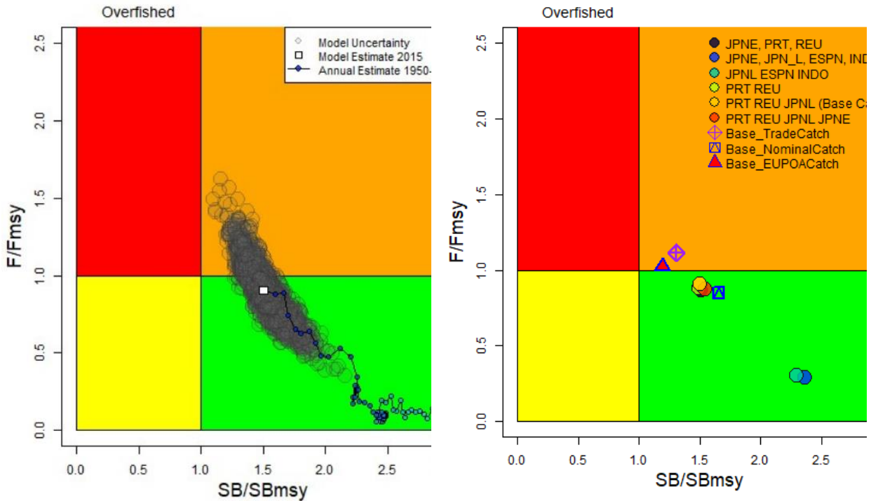
Fig. 1. Blue shark: Aggregated Indian Ocean stock assessment Kobe plot for the 2017 estimate based on the base case model and a range of sensitivity models explored with several catch reconstructions and fits to CPUE series. (Left panel: base case model with trajectory and MCMC uncertainties in the terminal year; Right panel: terminal year estimates of the sensitivity model runs). All models shown are run using SS3 - Stock Synthesis III.
