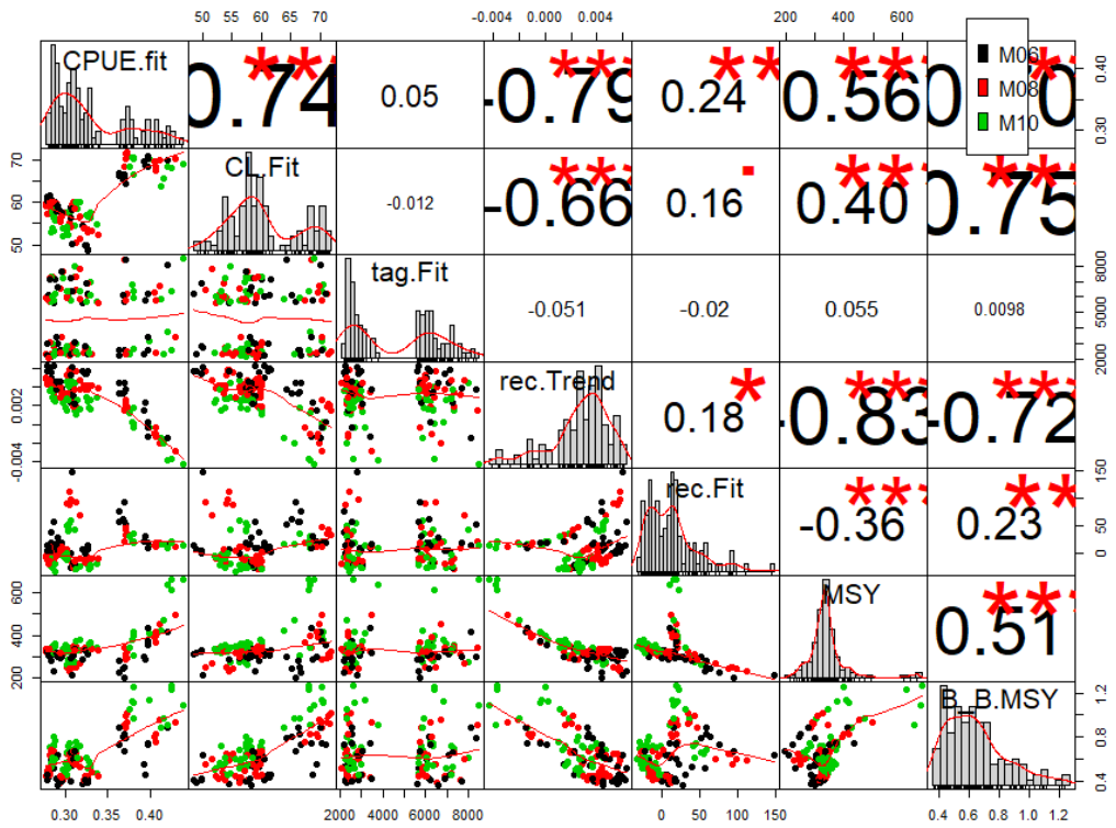
Figure 23. Multiway comparison of OMrefY20.1 model characteristics, partitioned by assumption by colour.
