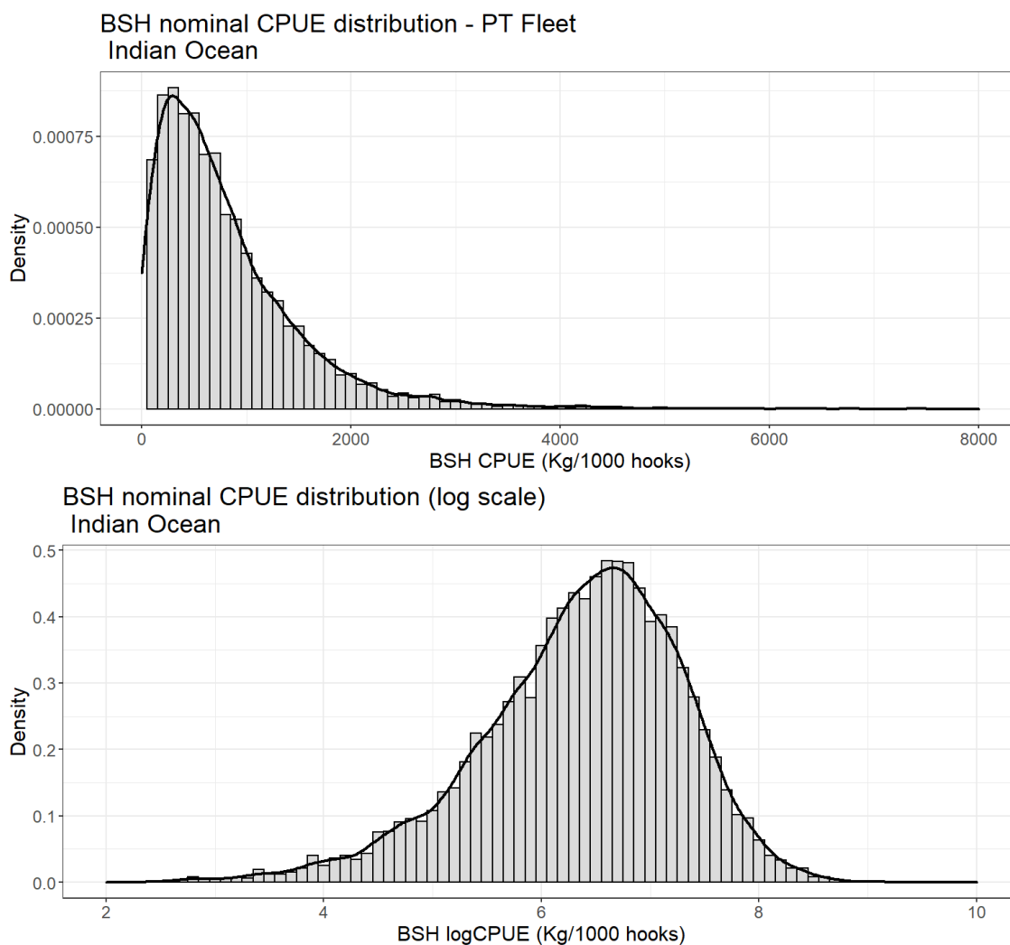
Figure 6: Distribution of the nominal blue shark CPUE captured by the Portuguese longline fleet in the Indian Ocean in non-transformed (top) and log-transformed (bottom) scales.
