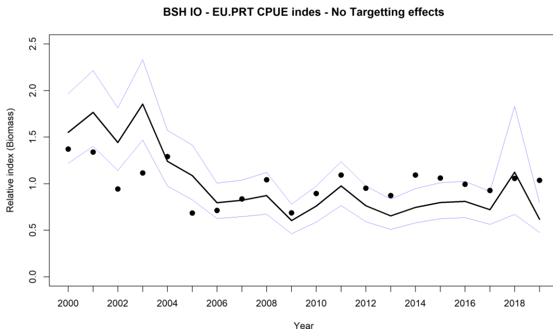
Figure 11. Standardized CPUE series for BSH captured by the Portuguese pelagic longline fleet in the Indian Ocean using a lognormal GLMM for the sensitivity model without targeting effects. The black line refers to the standardized index, the blue lines to the 95% confidence interval and the black dots to the nominal CPUE series.
