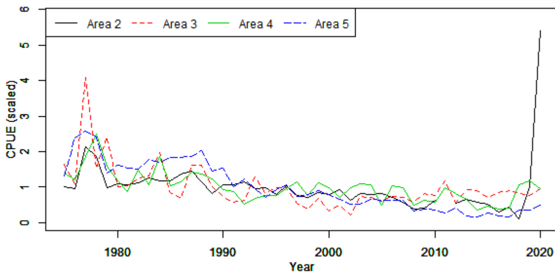
Fig. 6. Standardized year based CPUE in number for each area.
