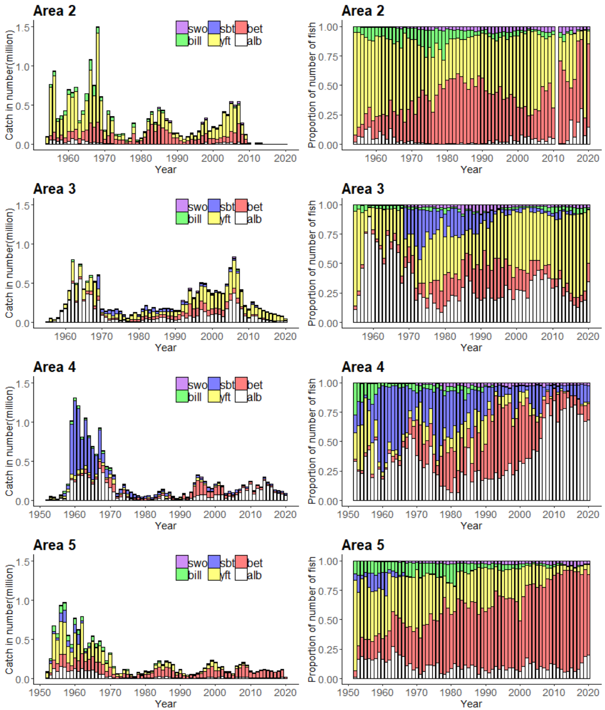
Fig. 3. Species composition of catch in number in the Indian Ocean by the Japanese longline fishery in each area shown in Fig. 1.
