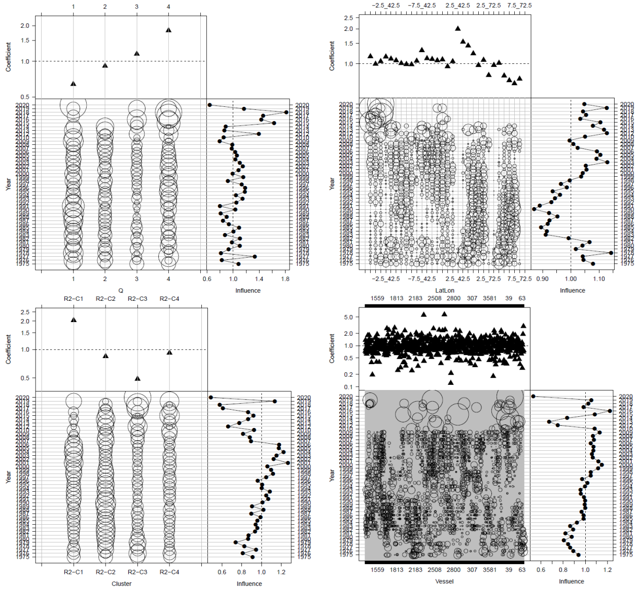
Fig. 9. Influence plot for CPUE standardization for yellowfin.
