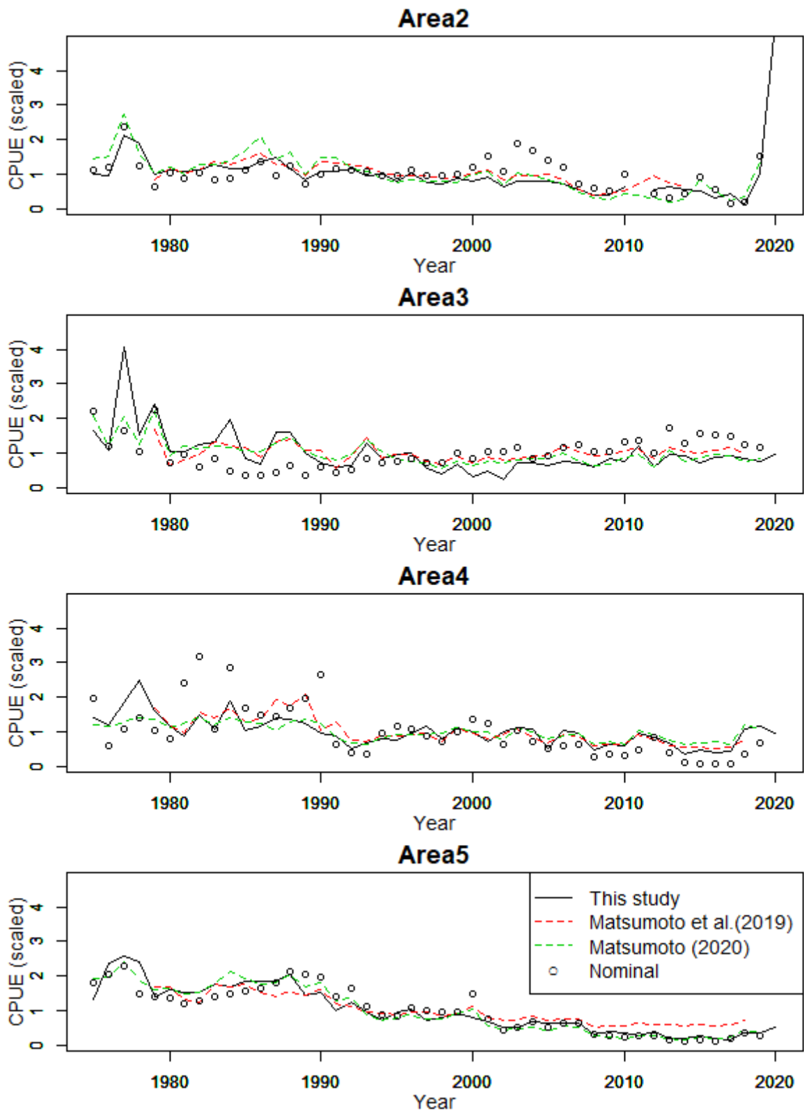
Fig. 7. Standardized year based CPUE in number for each area with comparison of nominal CPUE and CPUE in the previous studies (Matsumoto et al., 2019 and Matsumoto, 2020).
