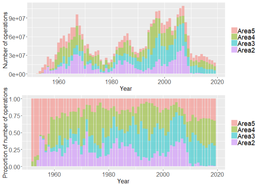
Fig. 2. Historical change in the proportion of fishing effort (number of hooks) in each area (Fig. 1).
