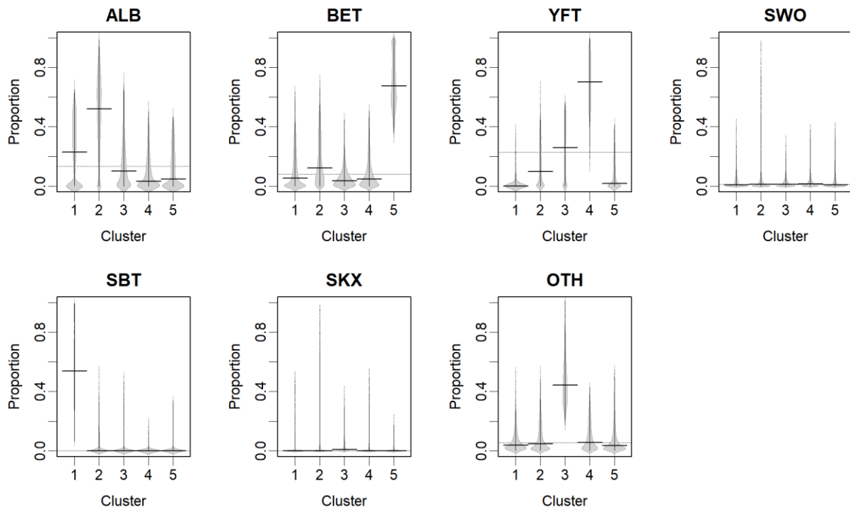
Fig. 4. Beanplots for yellowfin region showing species composition by cluster for albacore (ALB), bigeye tuna (BET), yellowfin tuna (YFT), swordfish (SWO), southern bluefin tuna (SBT), sharks (SKX) and other fish (OTH). The horizontal bars indicate the medians.
