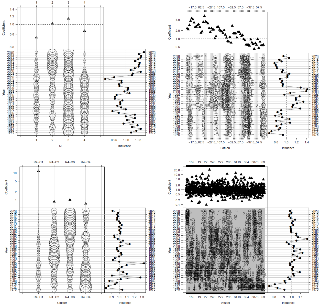
Fig. 9. Influence plot for CPUE standardization for yellowfin. (continued)
