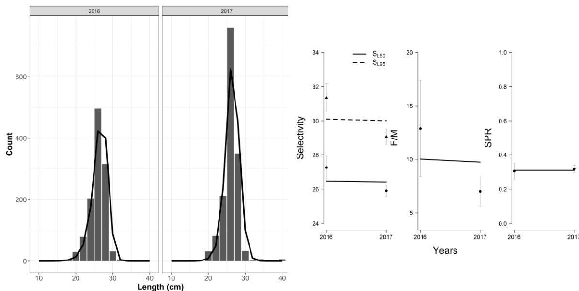
Figure 7: Results of LB-SPR method applied to the length samples from the gillnet fishery for bullet tuna: Fits to the length frequency in 2016 and 2017 (black dots) a; right – estimates ( with 95% CI) of logistic selectivity parameter ( a_{50} and a_{95} ), F/M, and Spawning Potential Ratio.
