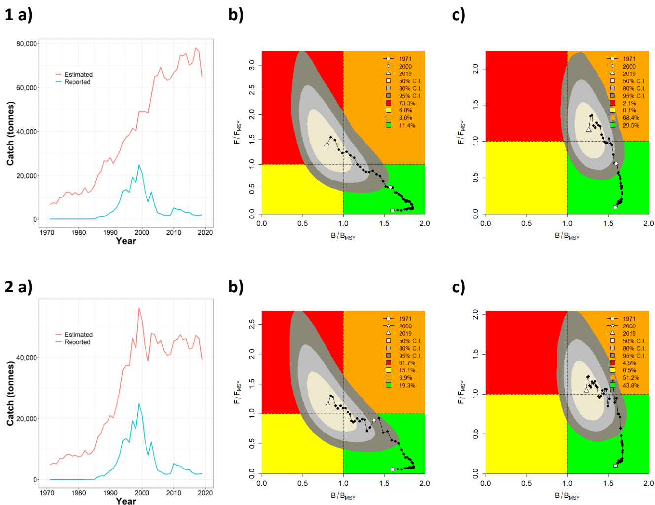
Figure 2. a) Reconstructed catch time series where the orange indicates estimated catch and blue indicates total reported silky shark catch; b) KOBE plots using r = low; c) KOBE plots using r = very low. The KOBE plots for each catch series reconstruction are displaying the change in biomass ( B ) and fishing mortality ( F ) relative to MSY ( B_{MSY} and F_{MSY} ) over time. The vertical line indicates B_{MSY} and the horizontal line indicates F_{MSY} . Grey areas represent confidence intervals (light grey = 50%, grey = 80%, and dark grey = 95%).
