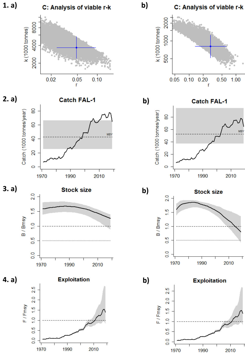
Figure 3. Diagnostic plots generated from CMSY for catch reconstruction 1. Figures on the left (a) show results using r = \text{very low} and figures on the right (b) show results using r = \text{low} . 1. Viable r - k pairs (grey dots) and best estimates with associated uncertainty (blue crosses). 2. Reconstructed catch time series (solid line) with estimated MSY value (dotted line) and associated confidence intervals (grey area). 3. Estimated stock biomass over time (solid line) with associated confidence intervals (grey area). Estimated B_{MSY} value (horizontal dotted line) and half of B_{MSY} (horizontal solid line). 4. Exploitation rate over time (solid line) with associated confidence intervals (grey area) and estimated F_{MSY} value (dotted line).
