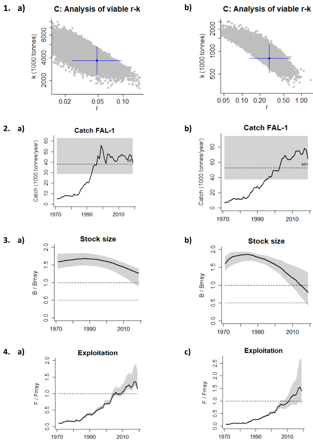
Figure 4. Diagnostic plots generated from CMSY for catch reconstruction 2. Figures on the left (a) show results using r = \text{very low} and figures on the right (b) show results using r = \text{low} . 1. Viable r - k pairs (grey dots) and best estimates with associated uncertainty (blue crosses). 2. Reconstructed catch time series (solid line) with estimated MSY value (dotted line) and associated confidence intervals (grey area). 3. Estimated stock biomass over time (solid line) with associated confidence intervals (grey area). Estimated B_{MSY} value (horizontal dotted line) and half of B_{MSY} (horizontal solid line). 4. Exploitation rate over time (solid line) with associated confidence intervals (grey area) and estimated F_{MSY} value (dotted line).
