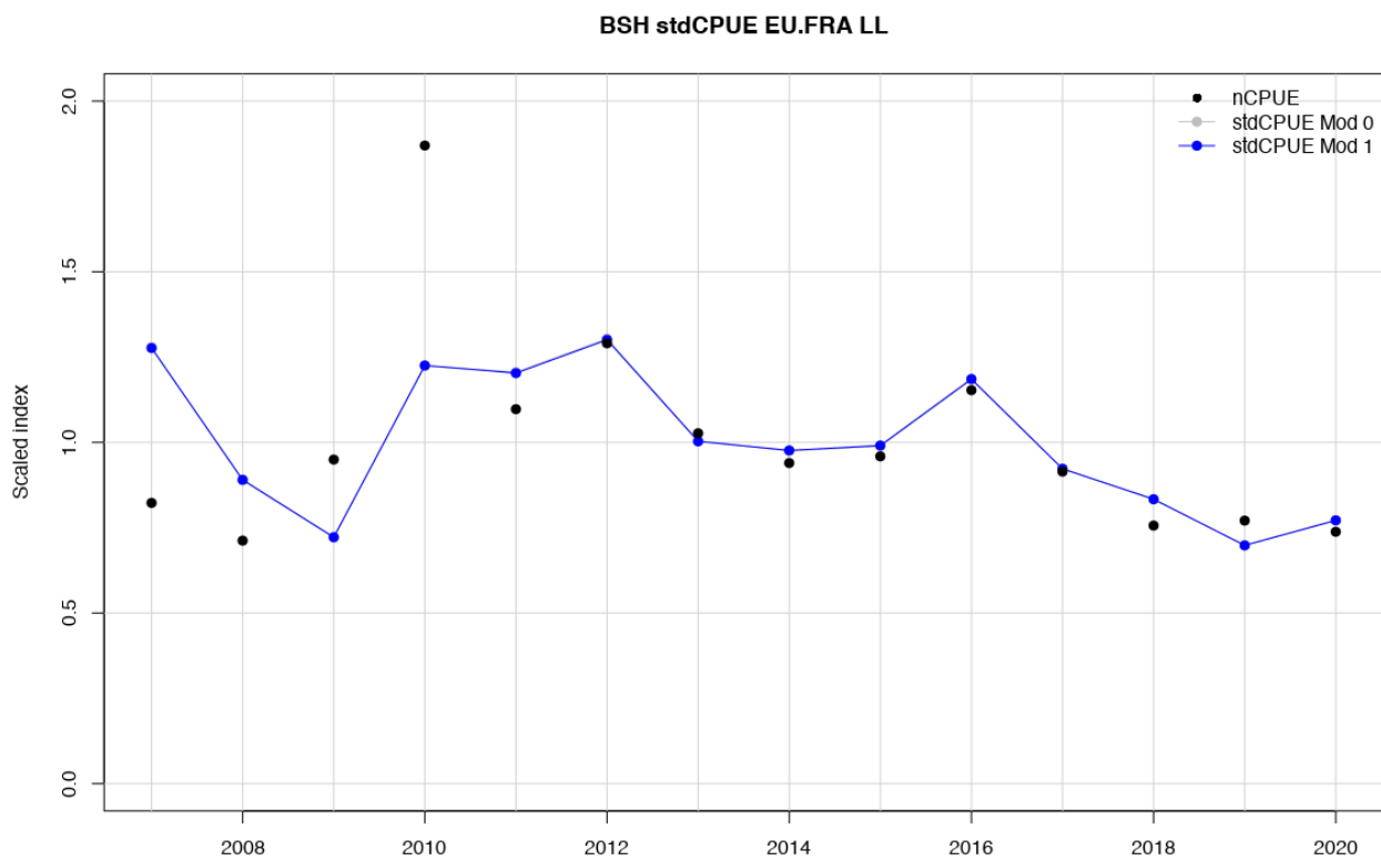
Figure 6. Scaled (by the mean) nominal and standardized CPUE time series of Mod 0 and Mod 1 for the French longline fishery based in Reunion Island (EU.FRA LL) for the period 2007-2020.
