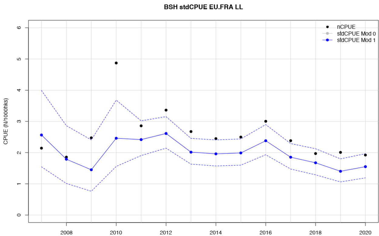
Figure 5. Nominal and standardized CPUE (N/1000 hooks) time series for Mod 0 and Mod 1 for the French longline fishery based in Reunion Island (EU.FRA LL) for the period 2007-2020.
