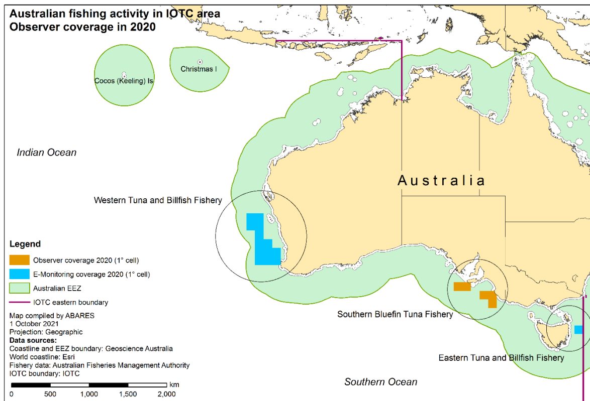
Figure 5 Spatial distribution of 2020 observer coverage in the longline fishery in the IOTC Area of Competence
