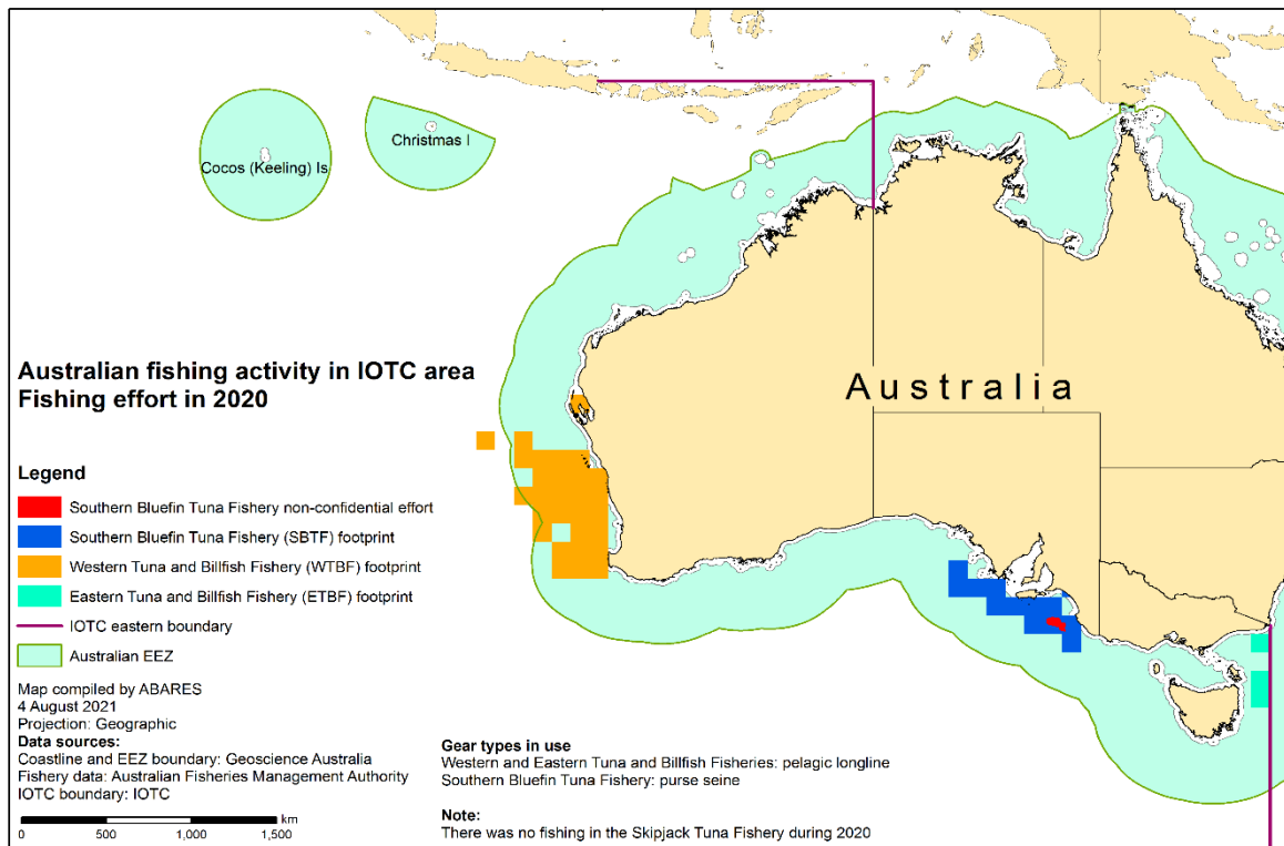
Figure 2a Fishing footprint (shown as 1-degree cells) in the WTBF and ETBF (longline) and in the SBTF (purse seine) for 2020
