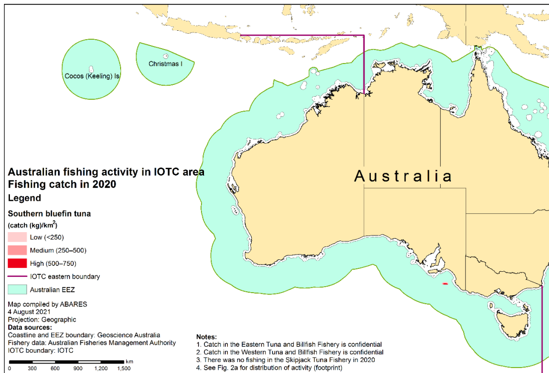
Figure 3a Distribution of catch in the SBTF (purse seine) for 2020. Note that due to the low effort in the longline fisheries, confidentiality rules prohibit the depiction of the 2020 WTBF and ETBF data
