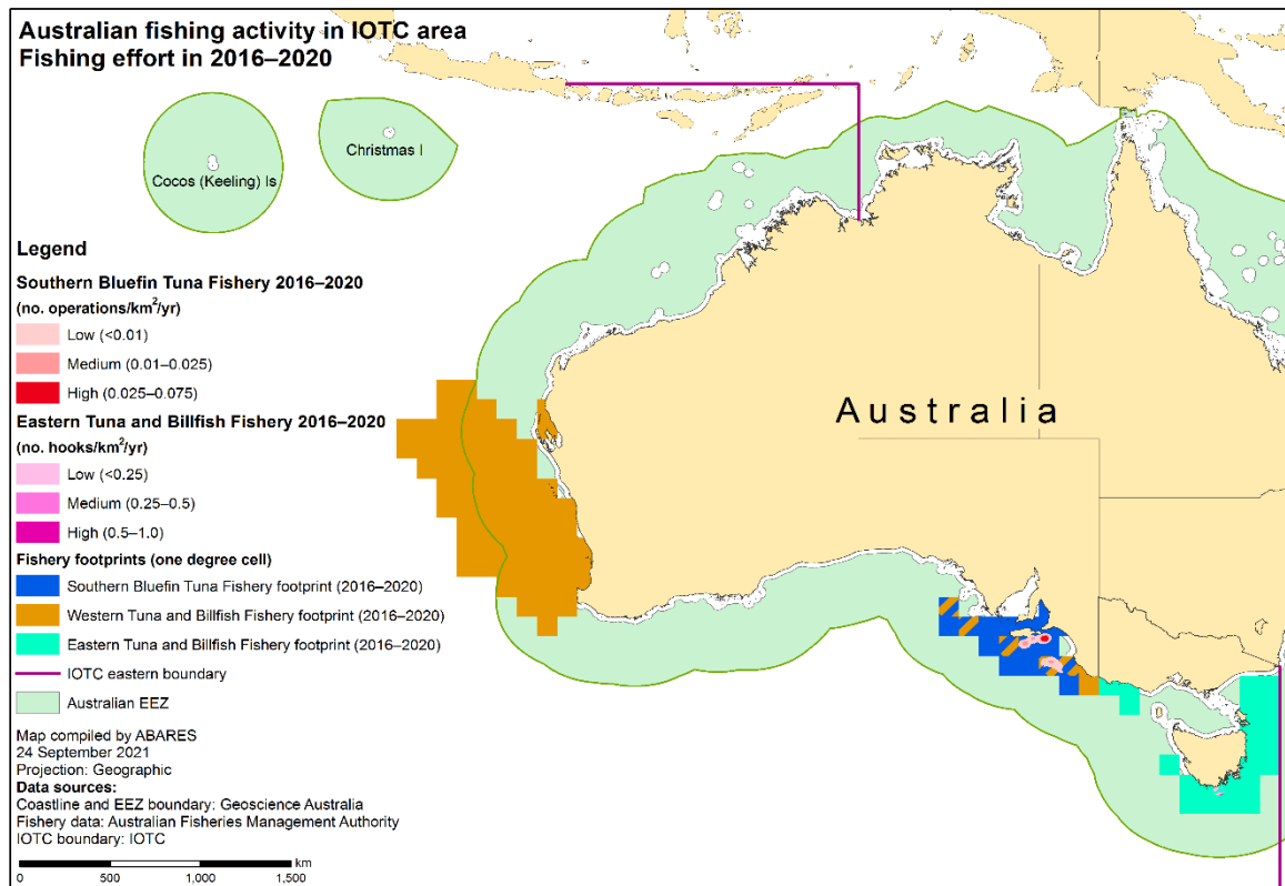
Figure 2b Aggregate fishing footprint (shown as 1-degree cells) in the WTBF and ETBF (longline) and in the SBTF (purse seine) for 2016 to 2020
