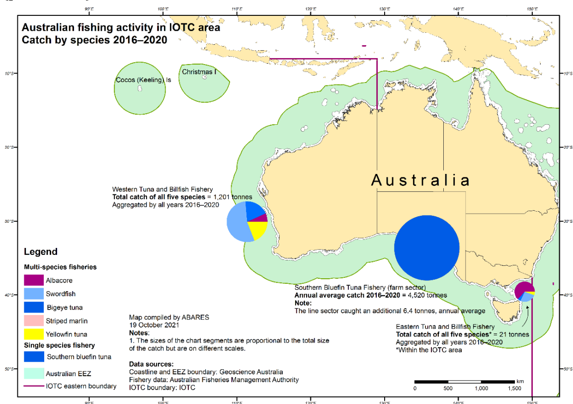
Figure 3b Distribution of catch in the WTBF (longline), ETBF (longline) and in the SBTF (purse seine) for 2016 to 2020
