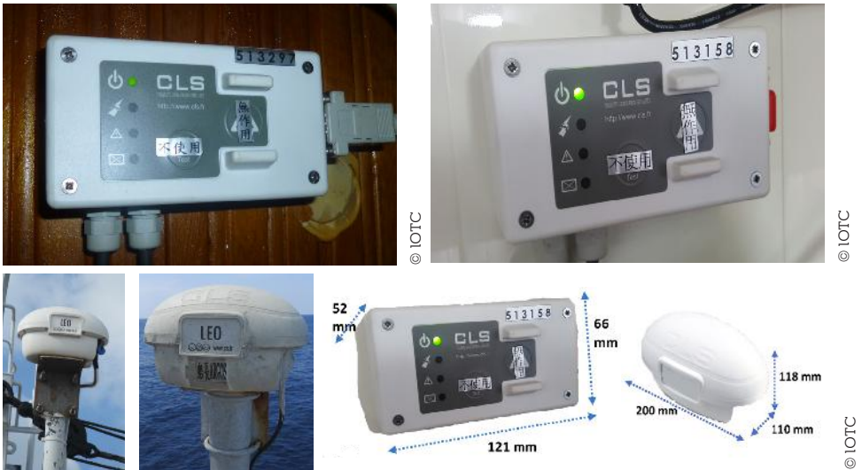
Figure 52: LEO unit and antenna
