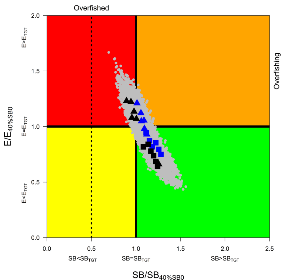
Fig. 2. Skipjack tuna: SS3 Aggregated Indian Ocean assessment Kobe plot of the 2020 uncertainty grid. Symbols represent MPD estimates of current stock status relative to SB 40%SB0 (x-axis) and E 40%SB0 (y-axis) for the individual models (blue, no effort creep; black, additional effort creep; triangle, full weighting of tagging data; square, tagging data downweighted). Grey dots represent uncertainty from individual models. The vertical dashed line represents the limit reference point for Indian Ocean skipjack tuna (SB lim = 20%SB 0 )
