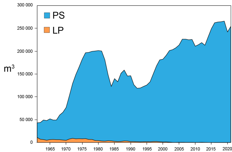
FIGURE 25. Carrying capacity, in cubic meters of well volume, of the purse-seine and pole and line fleets in the EPO, 1961-2021. Source: SAC-13-03 (Fig. 2).
