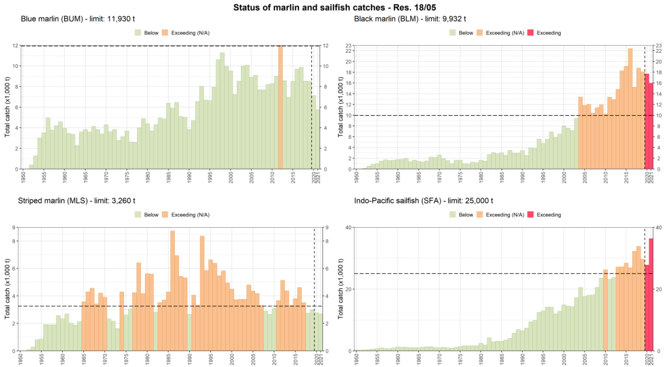
Figure 1: Status of marlin and sailfish catches in relation to the limits set out in Resolution 18/05. The horizontal dotted line indicates the catch limit while the vertical horizontal line indicates the period after which the limits apply
