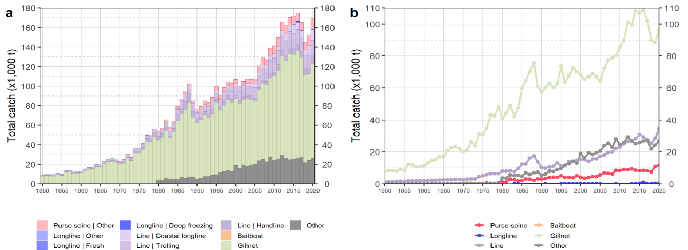
Fig. 2. Annual time series of (a) cumulative nominal catches (t) by fishery and (b) individual nominal catches (t) by fishery group for narrow-barred Spanish mackerel during 1950-2020
