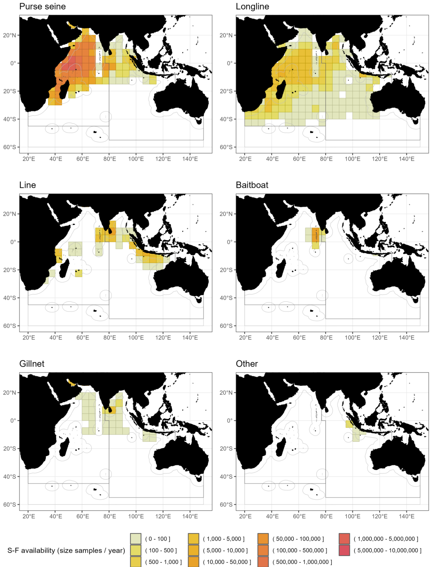
Figure 18: Spatial distribution (average number of samples per grid per year) of available yellowfin tuna size-frequency data for each fishery group in the period 2017-2021. Data source: standardized size-frequency dataset (Res. 15/02)
