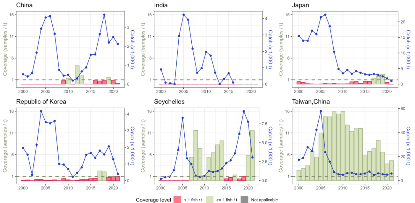
Figure 23: Size-frequency samples coverage (number of fish measured by t of retained catches) of yellowfin tuna caught by the major deep-freezing longline fleets, by fleet and year (2000-2021). Data source: standardized size-frequency dataset (Res. 15/02)
