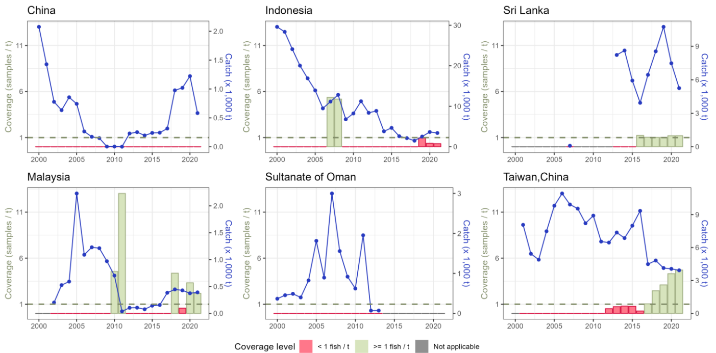
Figure 24: Size-frequency samples coverage (number of fish measured by t of retained catches) of yellowfin tuna caught by the major fresh-tuna longline fleets, by fleet and year (2000-2021). Data source: standardized size-frequency dataset (Res. 15/02)
