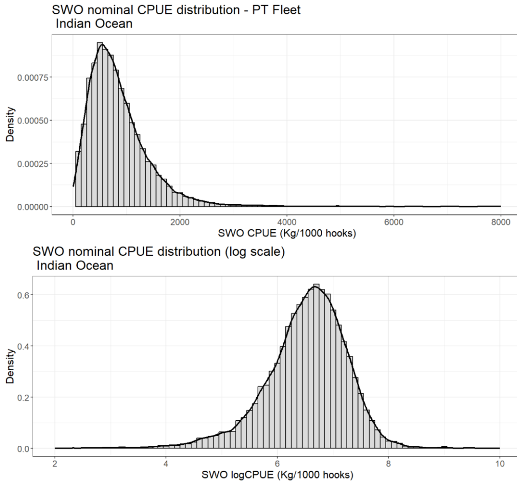
Figure 6: Distribution of the nominal swordfish CPUE captured by the Portuguese longline fleet in the Indian Ocean in non-transformed (top plot) and log-transformed (bottom plot) scales.
