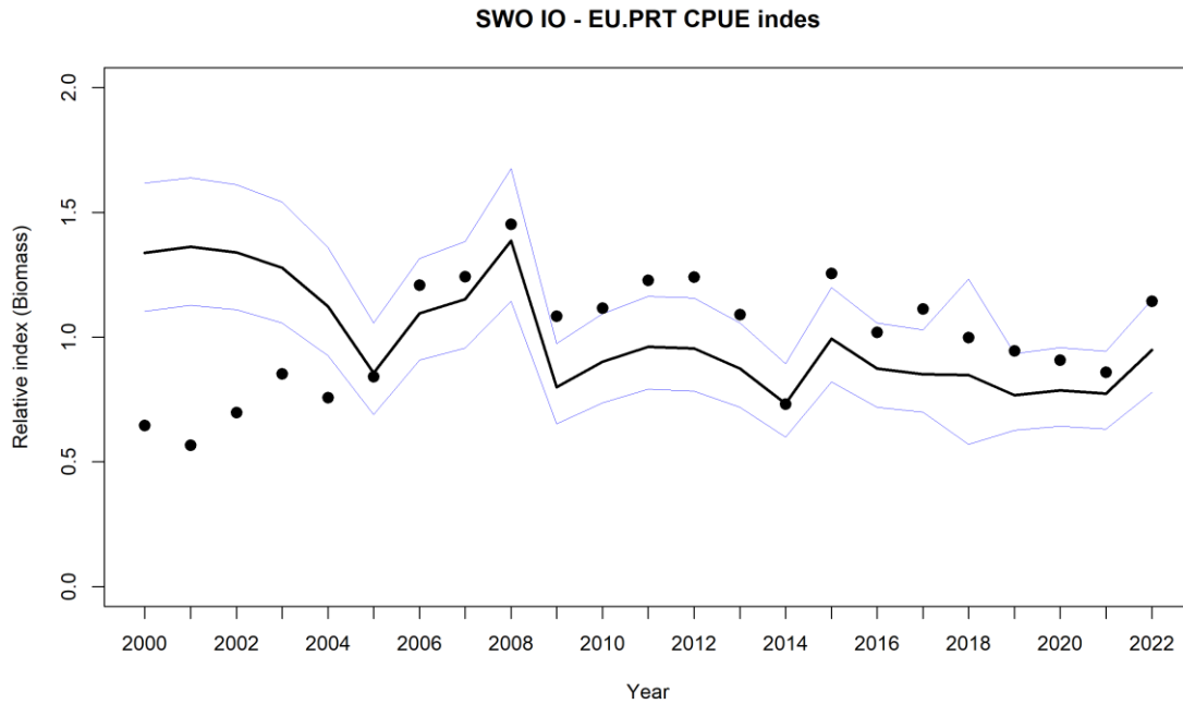
Figure 9. Standardized CPUE series for SWO captured by the Portuguese pelagic longline fleet in the Indian Ocean using a lognormal GLMM for the final selected model. The solid black line refers to the standardized index; solid blue lines refer to the 95% confidence intervals and the black dots to the nominal CPUE series.
