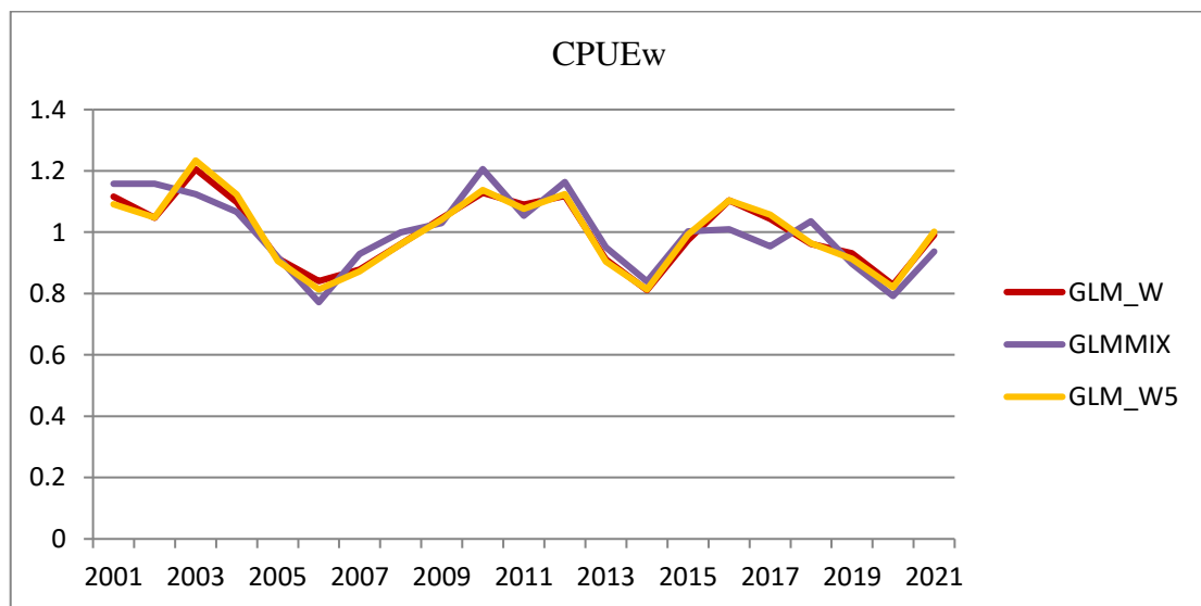
Figure 6. Comparative scaled standardized CPUE in number (upper panel) and in kg round weight (lower panel) for swordfish in the Indian Ocean for the period 2001-2021. Both series are scaled from their respective mean value. GLM_N/GLM_W: the base case in number/weight, GLM_N5/GLM_W5: the base case in number/weight with 5 categories of ratio factor, GLMMIX: the GLMM procedure in weight.
