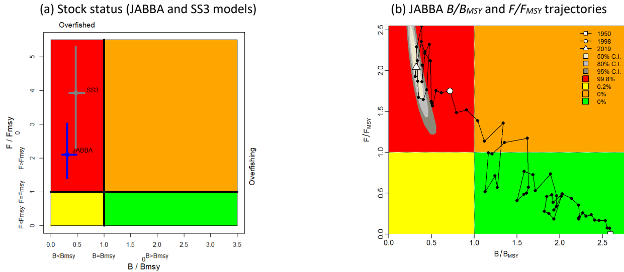
Fig. 3. (a) Striped marlin: Stock status from the Indian Ocean assessment JABBA (Bayesian State Space Surplus Production Model) and SS3 models with the confidence intervals (left); (b) Trajectories (1950-2019) of B/B_{MSY} and F/F_{MSY} from the JABBA model. NB: SS3 refers to SB/SB_{MSY} while the JABBA model's output refers to B/B_{MSY}
