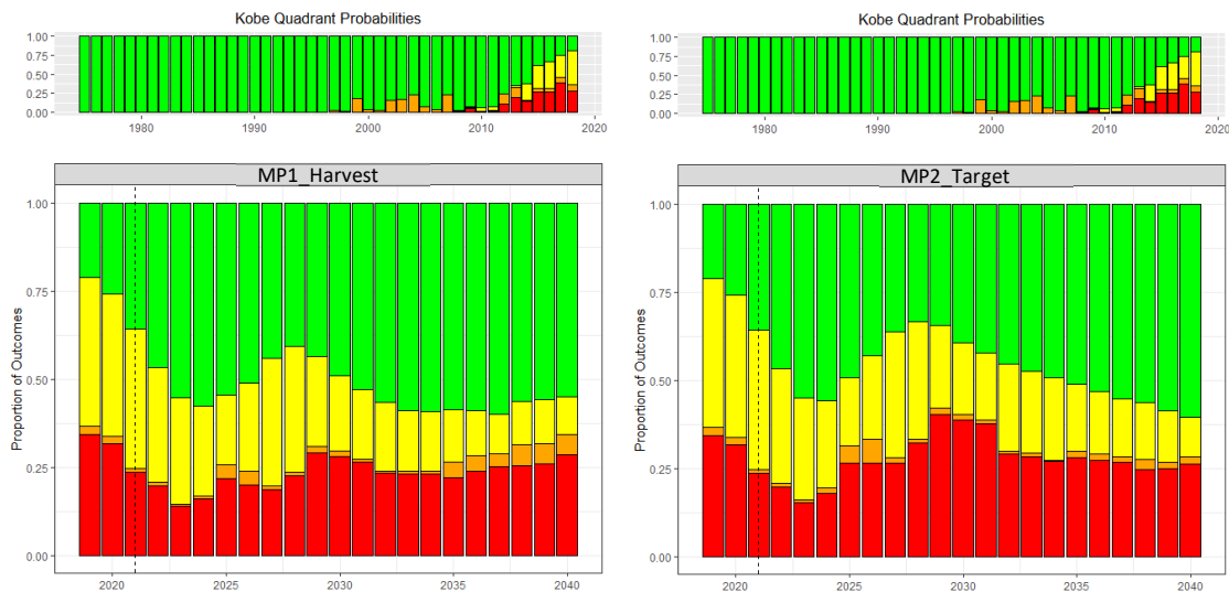
Figure C.5: Time-dependent Kobe probabilities for MP1_Harvest (left) and MP2_Target (right) for the recruitment shock robustness test.
