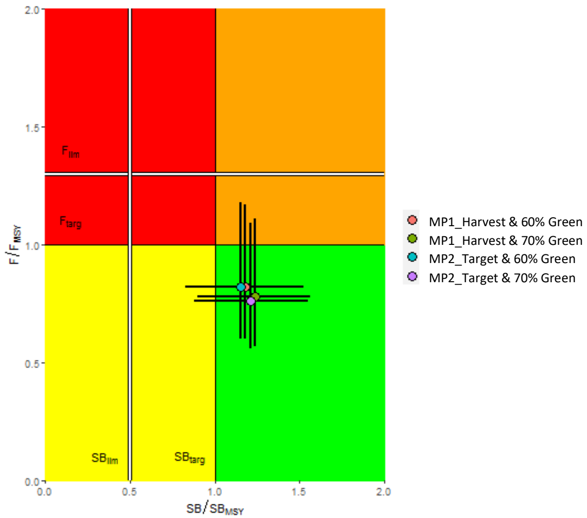
Figure C.3: Time-averaged Kobe plot for the two candidate MPs tuned to the 60% and 70% probability of being in the green zone of the Kobe plot during 2034-2038 and averaged over the first 20 years of the projection period, for the reference set. Error bars show the 80% confidence intervals.
