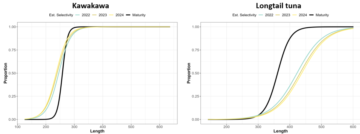
Figure 6 : Estimated selectivity curves for KAW and LOT from 2022 to 2024 based on LBSR analysis
