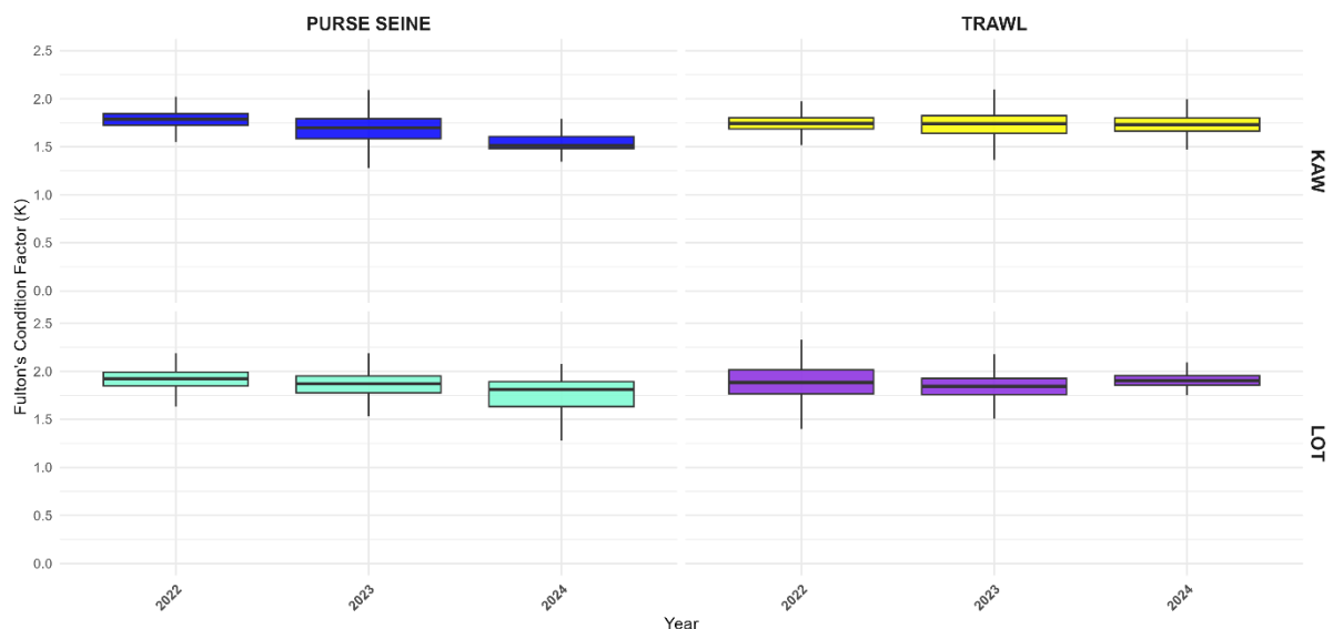
Figure 3 : Boxplot showing the distribution of condition factor (K) values for KAW and LOT sampled from the west coast of Peninsular Malaysia.
