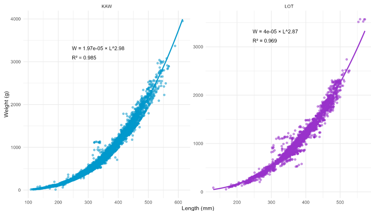
Figure 1 : Length-weight relationships of KAW and LOT from West Coast of Peninsular Malaysia
