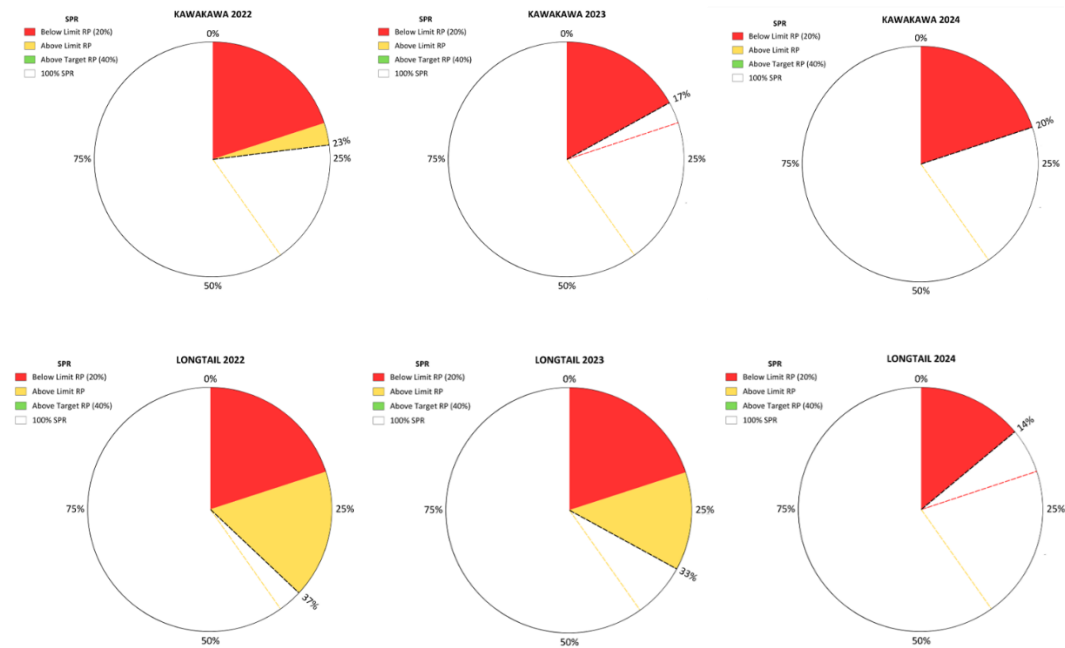
Figure 5 : Proportions of current spawning potential ratio (SPR) for KAW and LOT
