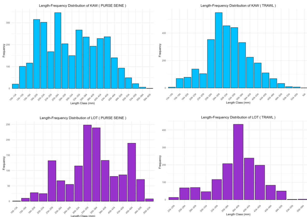
Figure 2 : Length frequency distribution of KAW and LOT
