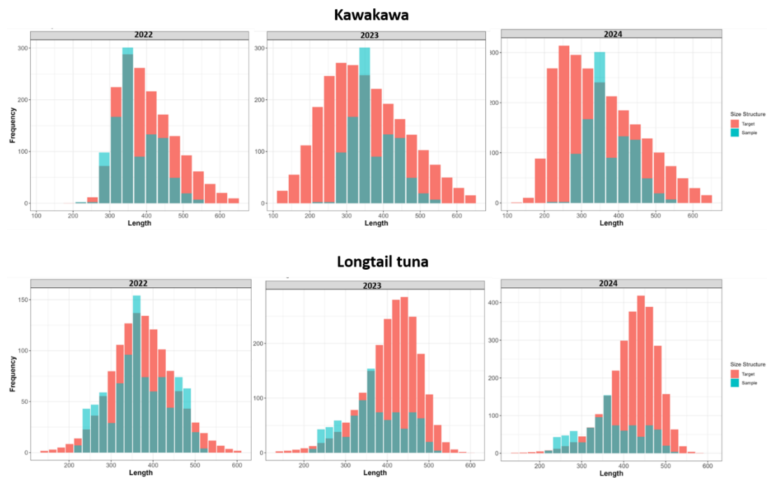
Figure 4 : Observed and theoretical size distribution of KAW and LOT under 40% SPR scenario
