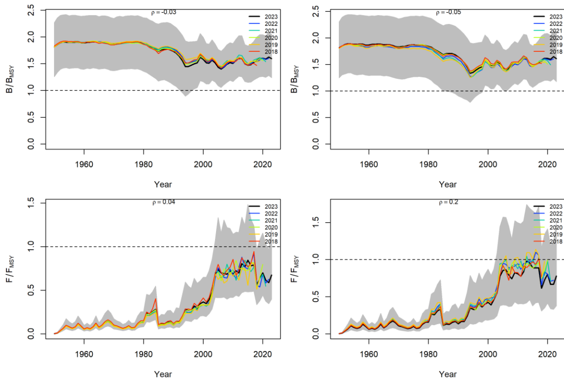
Figure A7. Retrospective analysis conducted for the final main base models developed for the IOTC blue shark stock assessment, by removing 1-year at a time sequentially ( n=5 ) and predicting the trends in biomass and fishing mortality relative to MSY (i.e., B/B_{msy} and F/F_{msy} ).
