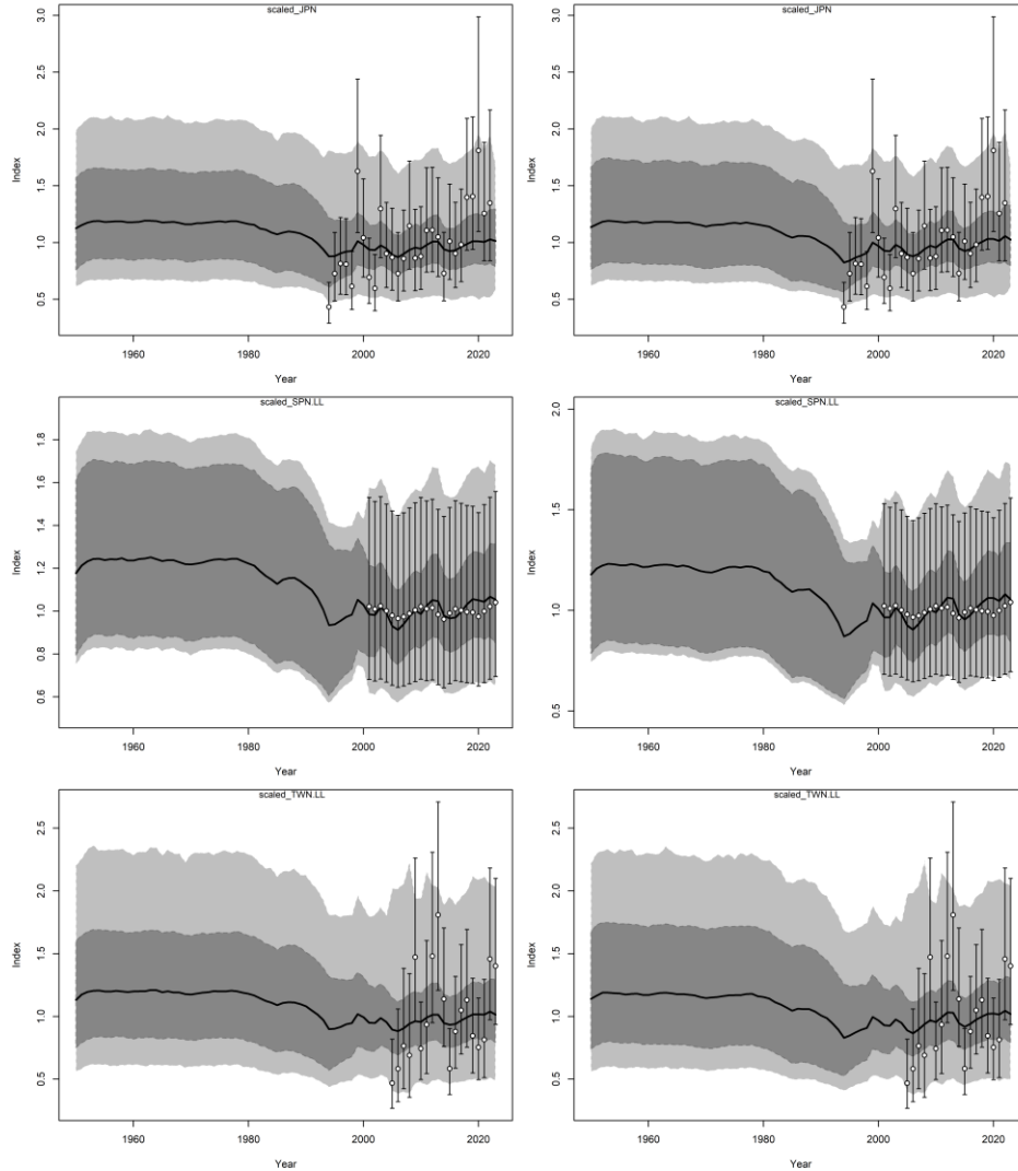
Figure A3. Time series of observed (circles) and predicted (solid line) CPUEs for the IOTC blue shark stock assessment models for the final base models. The dark shaded areas represent the 95% credibility intervals of the expected mean CPUE, and the light shaded areas represent the 95% posterior predictive distribution intervals. The error bars are the 95% confidence intervals (CIs) from the CPUE observations
