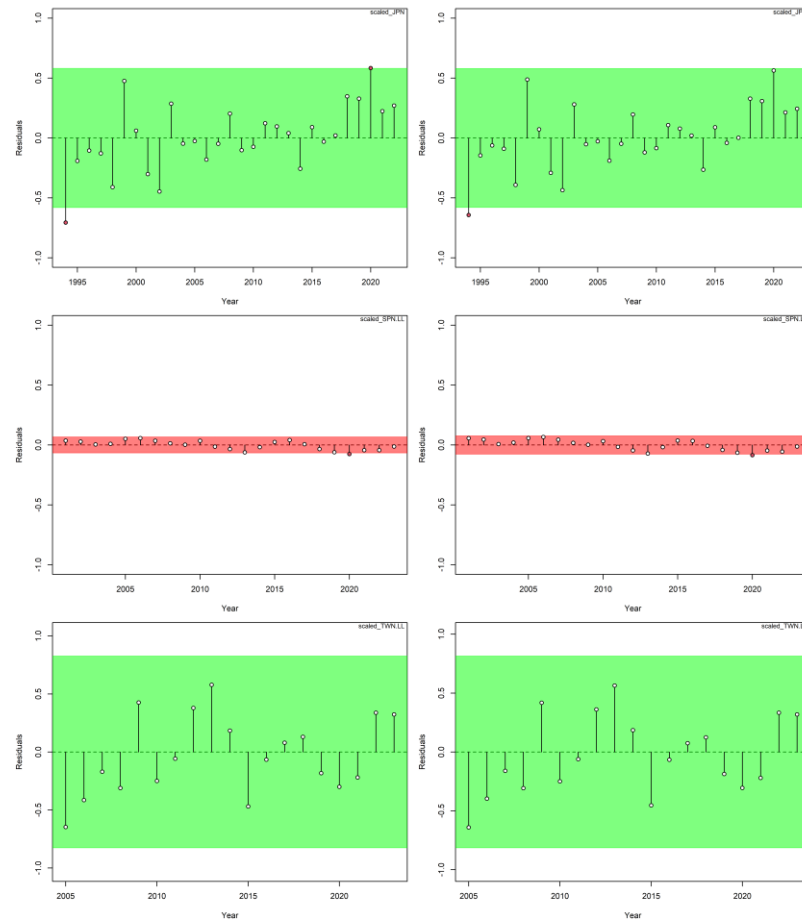
Figure A5. Runs tests for the CPUE index used for the final base models used in the IOTC blue shark stock assessment.
