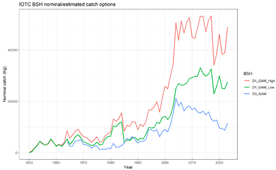
Figure A1: Selected time series of the IOTC BSH nominal and estimated catch data options that were finally considered for the base case (D1 GAM low) and sensitivities (D1 GAM High and D3 GAM).
