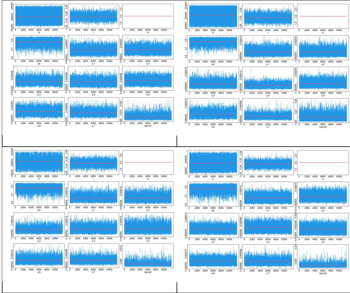
Figure 4: Trace plots of the base models used for the IOTC blue shark stock assessment.
