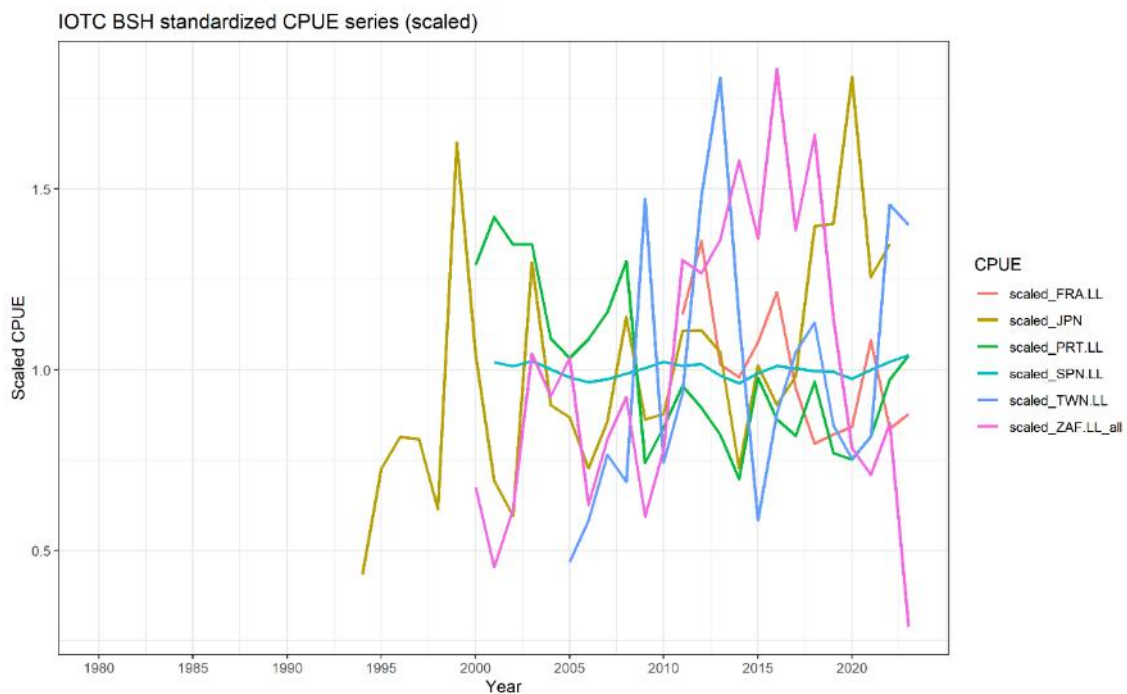
Figure A2: Standardized CPUE series used for the IOTC BSH stock assessment. For better visualization and comparison, each series is scaled by their respective means. The series were used either as the base case or as sensitivity analysis.
