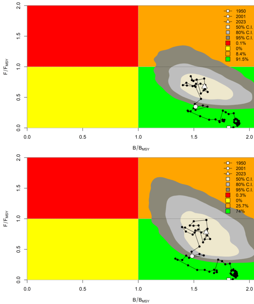
Figure A9. Kobe phase plot with the estimated trajectories (1950-2023) of B/B_{msy} and F/F_{msy} for the final base models considered for the 2025 IOTC blue shark stock assessment. The different grey shaded areas denote the 50%, 80%, and 95% credibility intervals for the terminal year of the assessment data (2023). The probability of the terminal year stock status falling within each quadrant of the Kobe phase plot is indicated in the figure legend, for each of the grid models.
