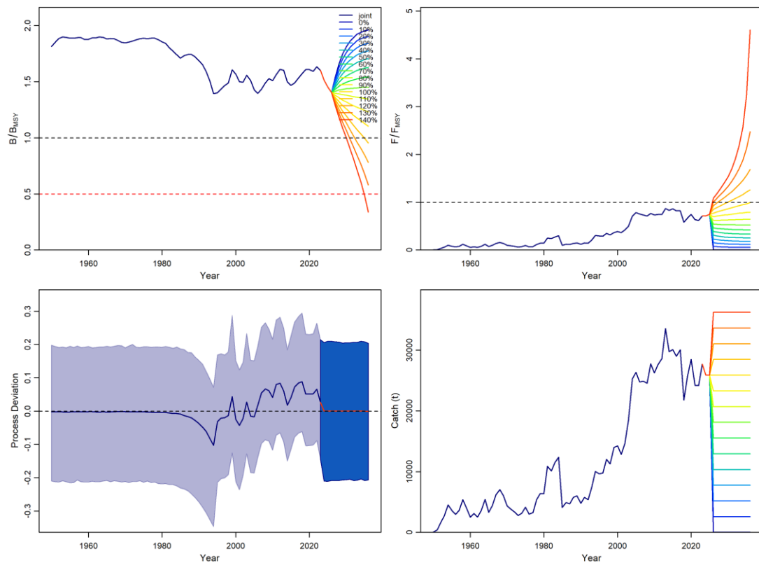
Figure A10. Projections from the 2 final agreed models used for the stock assessment of the blue shark in IOTC, carried out in 2025.
