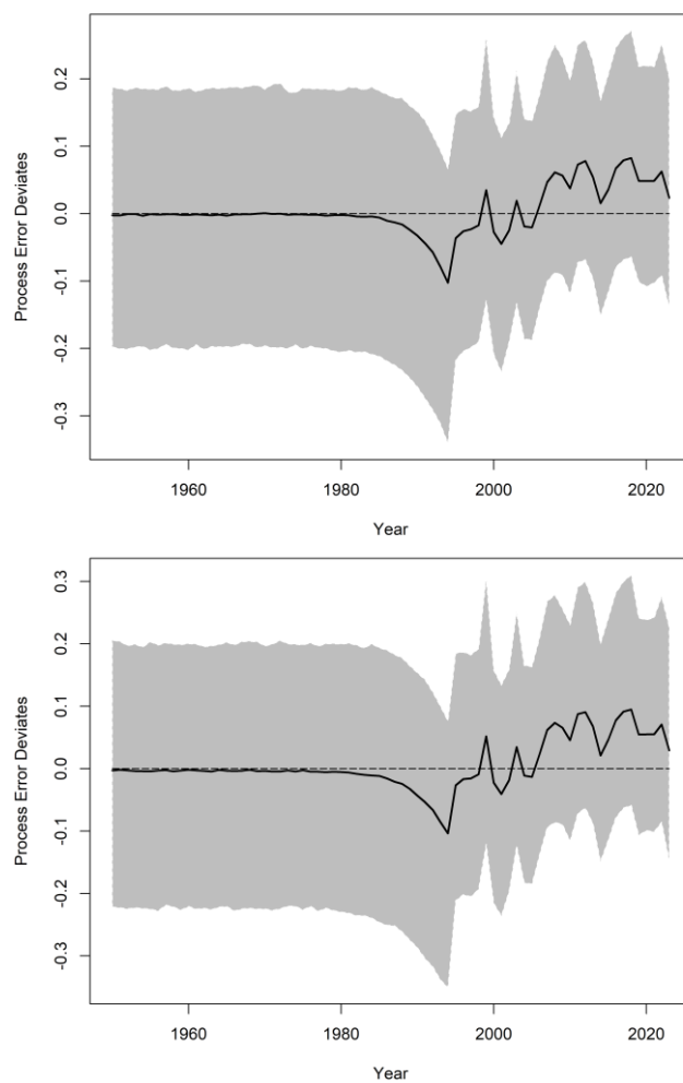
Figure A6. Process error deviates from the final main base models used for the IOTC blue shark stock assessment. The solid line represents the median, and the shaded gray area the 95% credibility intervals.
