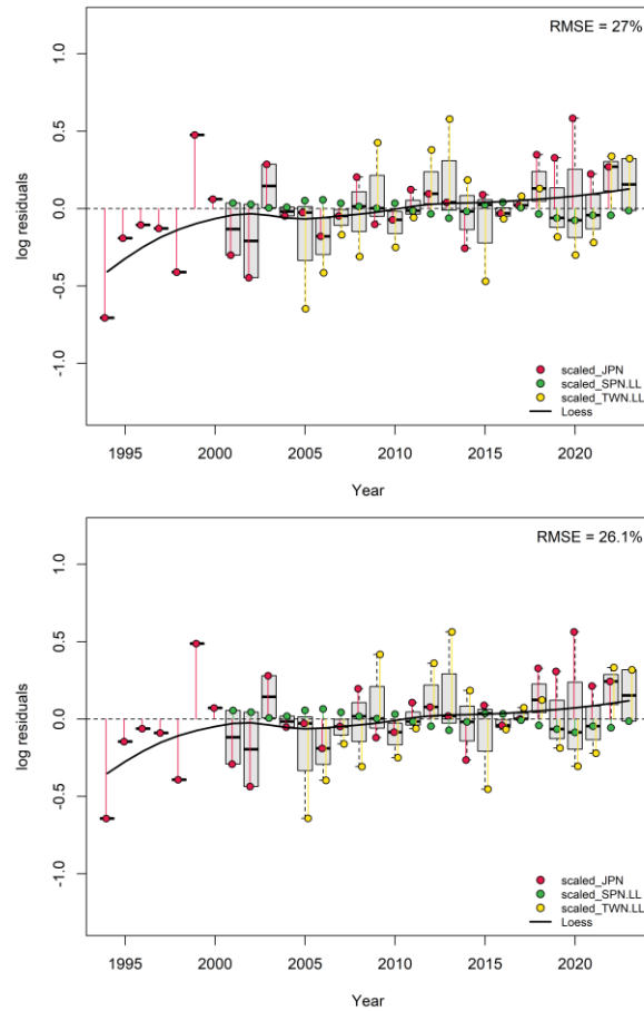
Figure A4. Final residuals diagnostic plots for the base models used for the IOTC blue shark stock assessment. Each individual CPUE index and its respective residuals are represented by a different color. The solid black lines represent loess smoothers through all residuals combined.
