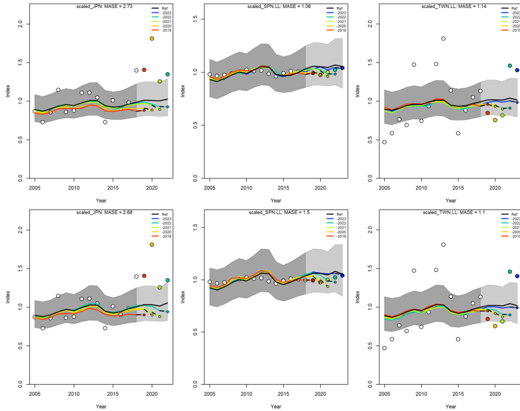
Figure A8. Hindcasting cross-validation results for the final indices used in the final models, available in the last years of the model, run for the final base models. The plots show 1-year-ahead forecasts of CPUE values, when the last years are removed one at a time, relative to the observed CPUE using all data. The CPUE observations, used for cross-validation are highlighted as the color-coded solid circles with associated light-grey shaded 95% confidence interval.
