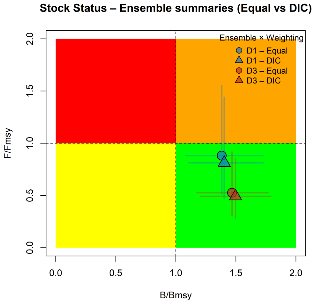
Figure 22. Kobe plot with the point estimates and CIs of the summarized large grid models, using two options for model weighing: 1) equal weights across all models; 2) using DIC-weights across models, and the 2 ensemble grids (based on D1 and D3 catches). The summaries are done with all the grid models that have converged.
