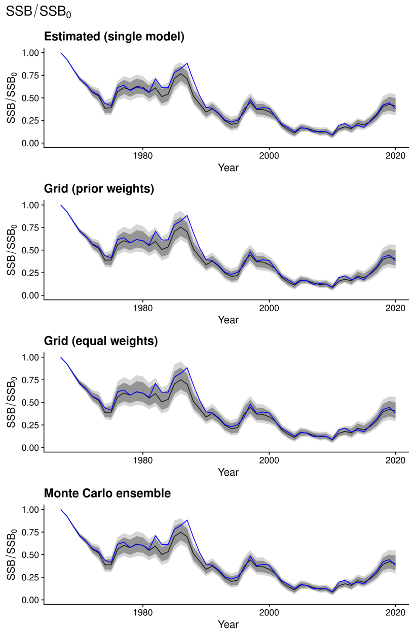
Figure B-2: Time series of stock status: (SSB: spawning stock biomass relative to SSB 0 : unfished spawning biomass) for four assessment approaches using estimated productivity (filled dark blue), bootstrap Monte Carlo (MC) draws from a productivity prior (light-blue), and prior-weighted and equal-weight factorial uncertainty grids over the productivity prior. All methods use the same productivity prior, which is centered on the true value with a low CV (10%). Solid lines indicate the median across ensembles (or the posterior median for the estimated case). The true simulated time-series is shown by the dark blue line.
