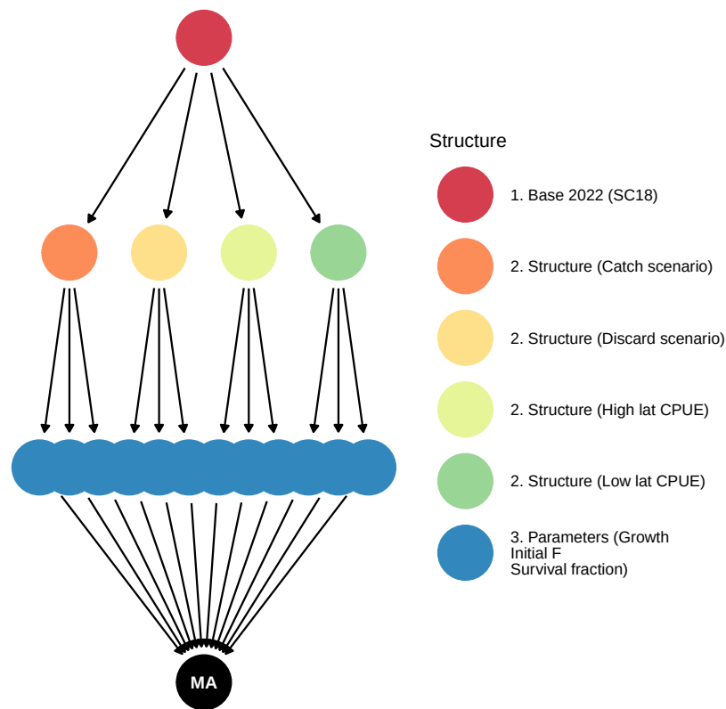
Figure 9: Examples of the 2022 South Pacific Blue Shark stock assessment grid, represented as hypothesis trees, separating structural and parameter uncertainty, and indicating which were used for management advice.
