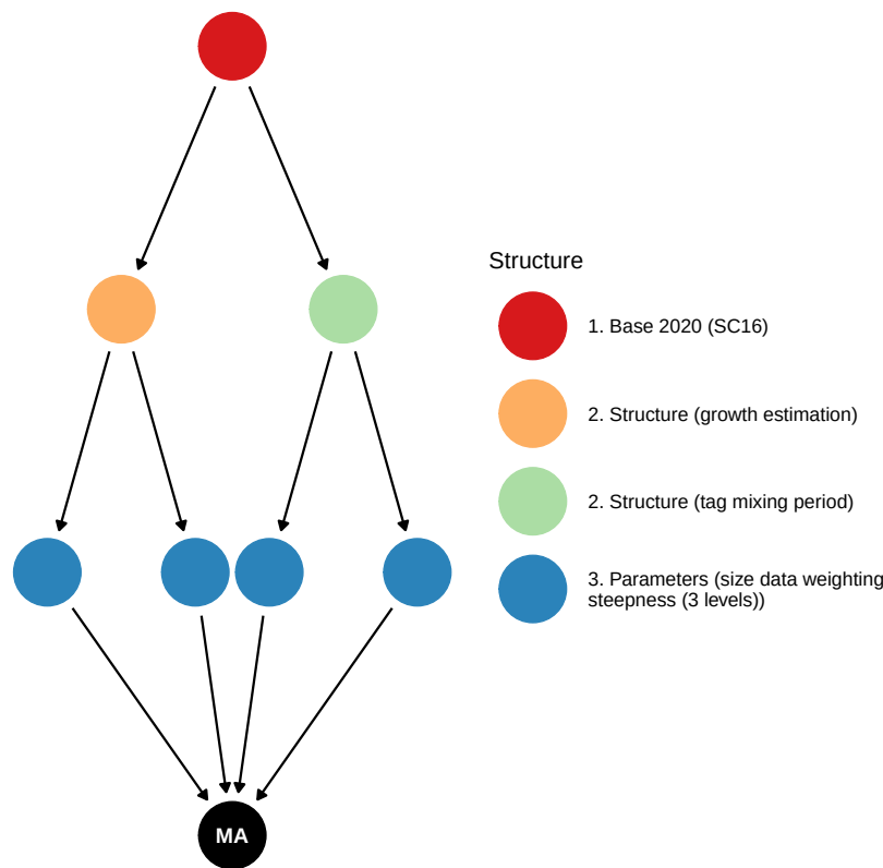
Figure 8: Examples of the 2021 Yellowfin tuna stock assessment grid, represented as hypothesis trees, separating structural and parameter uncertainty, and indicating which were used for management advice.
