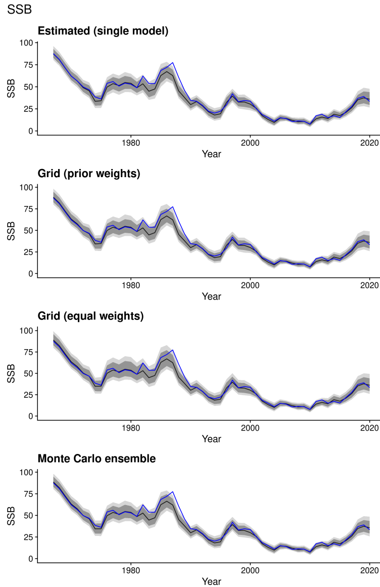
Figure B-1: Time series of spawning stock biomass SSB for four assessment approaches using estimated productivity (filled dark blue), bootstrap Monte Carlo (MC) draws from a productivity prior (light - blue), and prior - weighted and equal - weight factorial uncertainty grids over the productivity prior. All methods used the same productivity prior, which was centred on the true value with a low coefficient of variation (10%). Solid lines indicate the median across ensembles (or the posterior median for the estimated case). The true simulated time series is shown by the dark blue line.
