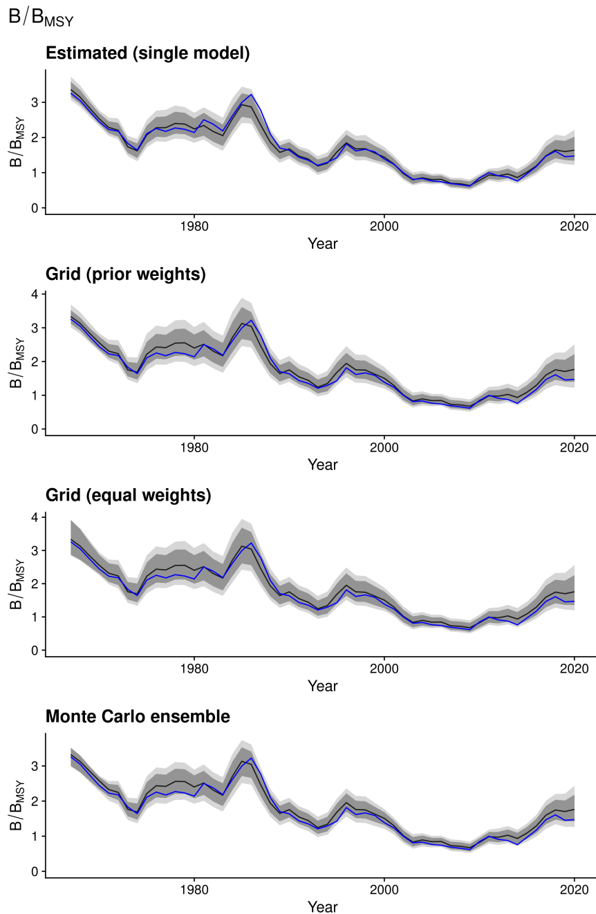
Figure B-11: Time series of stock status relative to MSY: (spawning stock biomass (SSB) relative to SSB that produces maximum sustainable yield (MSY)) for four assessment approaches using estimated productivity (filled dark blue), bootstrap Monte Carlo (MC) draws from a productivity prior (light-blue), and prior-weighted and equal-weight factorial uncertainty grids over the productivity prior. All methods use the same productivity prior, which is biased high by 0.05 for both parameters relative to the true value, with a tight prior (CV 10%) representing seemingly good understanding of productivity. Solid lines indicate the median across ensembles (or the posterior median for the estimated case). The true simulated time-series is shown by the dark blue line.
