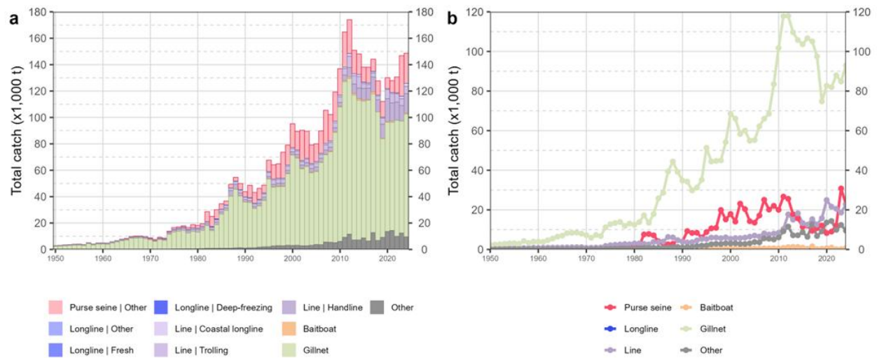
Fig. 2. Annual time series of (a) cumulative nominal catches (t) by fishery and (b) individual nominal catches (t) by fishery group for longtail tuna during 1950-2024
