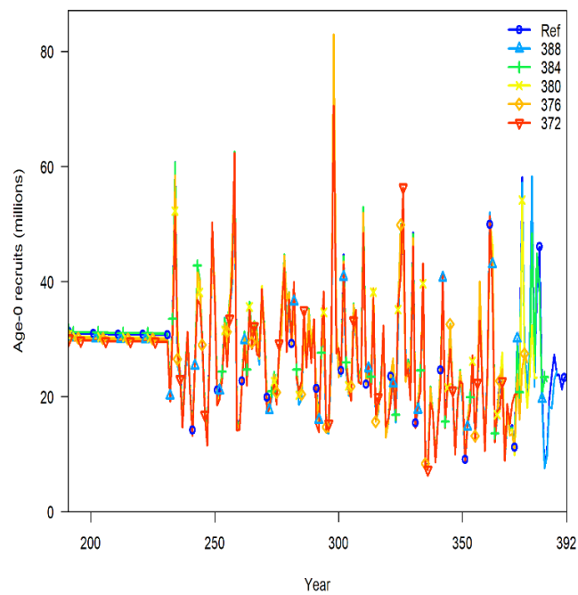
Figure 32: Retrospective analysis summary for recruitment estimates from the base model '6_update_bias'.
