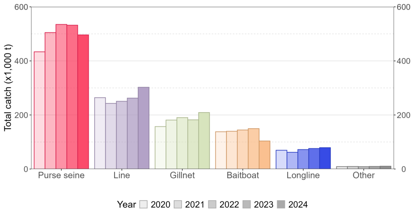
Figure 6: Annual catch (metric tonnes; t) trends of Indian Ocean tropical tuna by fishery group between 2020 and 2024
