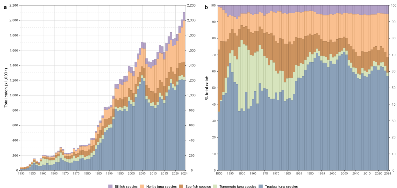
Figure 1: Annual time series of cumulative absolute (a) and relative (b) catches (metric tonnes; t) of all IOTC tuna and tuna-like species by species category for the period 1950-2024
