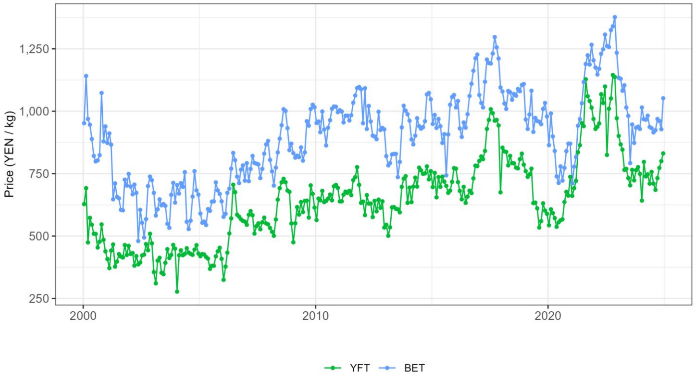
Figure 19: Monthly time series of import prices (YEN/kg) in Japan for sashimi-grade frozen during the period 2000-2024. Data sourced from Japanese customs, compiled, and curated by the FFA Fisheries Development Division (Ruaia et al. 2020)
