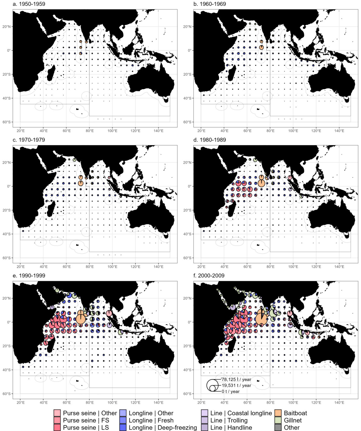
Figure 14: Estimated mean annual time-area catches (metric tonnes; t) of Indian Ocean tropical tuna by decade, 5°x5° grid, and fishery. Data source: tropical tuna raised time-area catches
