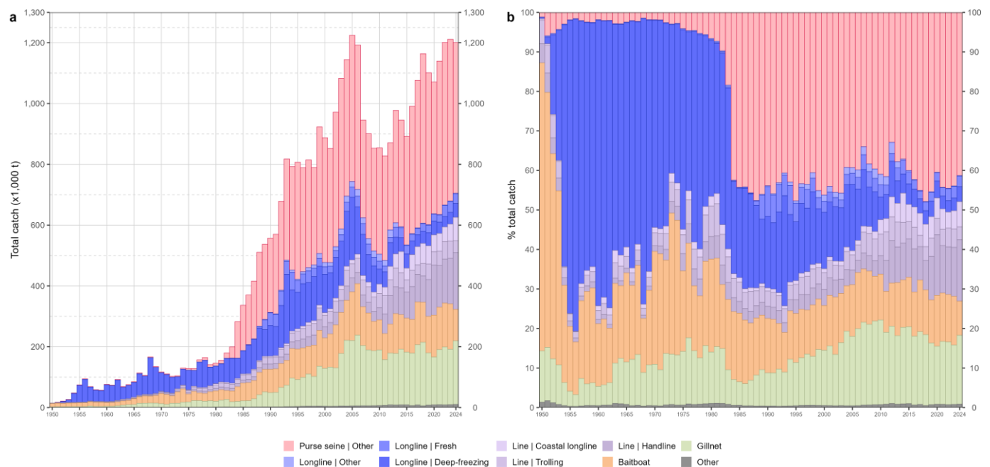
Figure 4: Annual time series of retained catches (metric tonnes; t) of Indian Ocean tropical tuna by fishery for the period 1950-2024
