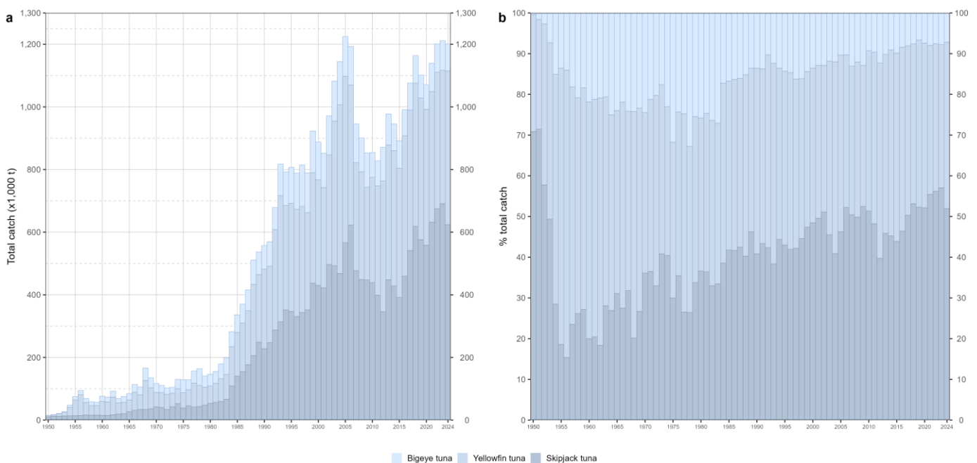
Figure 3: Annual time series of cumulative retained absolute (a) and relative (b) catches (metric tonnes; t) of Indian Ocean tropical tuna by species for the period 1950-2024
