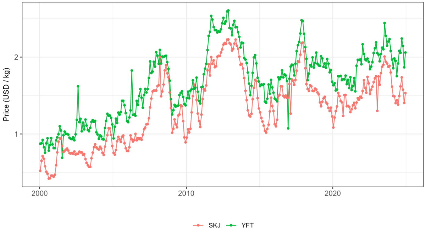
Figure 18: Monthly time series of import prices (USD/kg) in Thailand for canning-grade frozen skipjack and yellowfin tunas during the period 2000-2024. Data sourced from Thailand customs, compiled, and curated by the FFA Fisheries Development Division (Ruaia et al. 2020)
