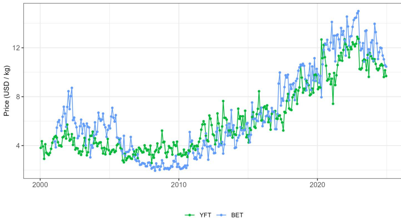
Figure 21: Monthly time series of import prices (USD/kg) in Thailand for canning-grade frozen during the period 2000-2024. Data sourced from USA customs, compiled, and curated by the FFA Fisheries Development Division (Ruaia et al. 2020)
