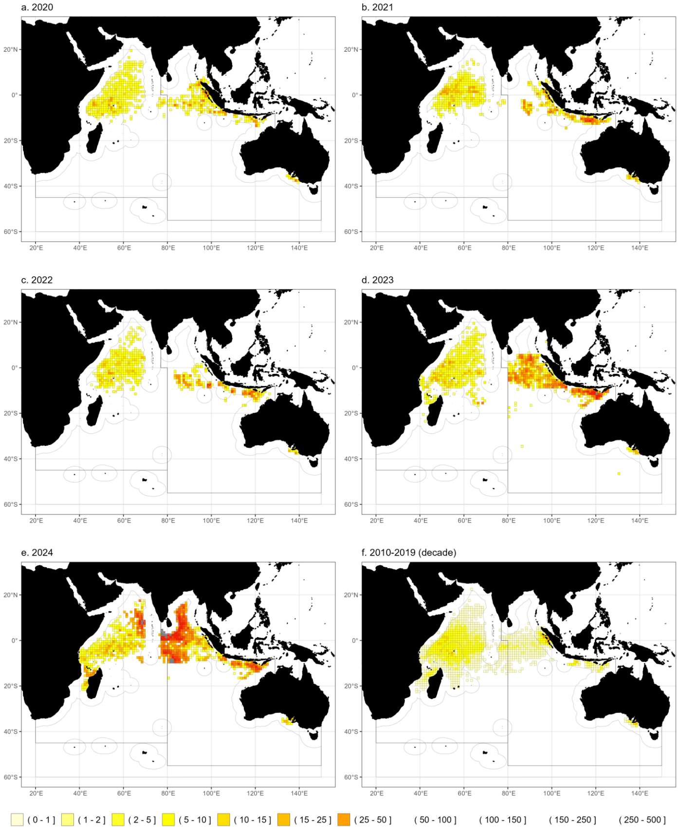
Figure 13: Mean annual effort (fishing days) exerted by purse seine fleets from other flags (OT) by year / decade and 1°x1° grid. Data source: time-area effort dataset for purse-seine fisheries (Res. 15/02)
