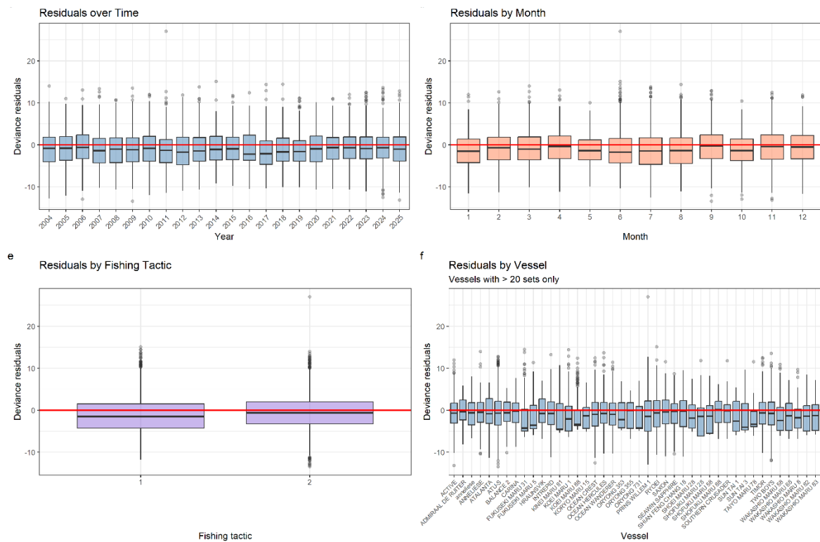
Figure 7. Residual plots of the tweedie standardisation showed no systematic patterns across years, months, vessels, or fishing target categories.
