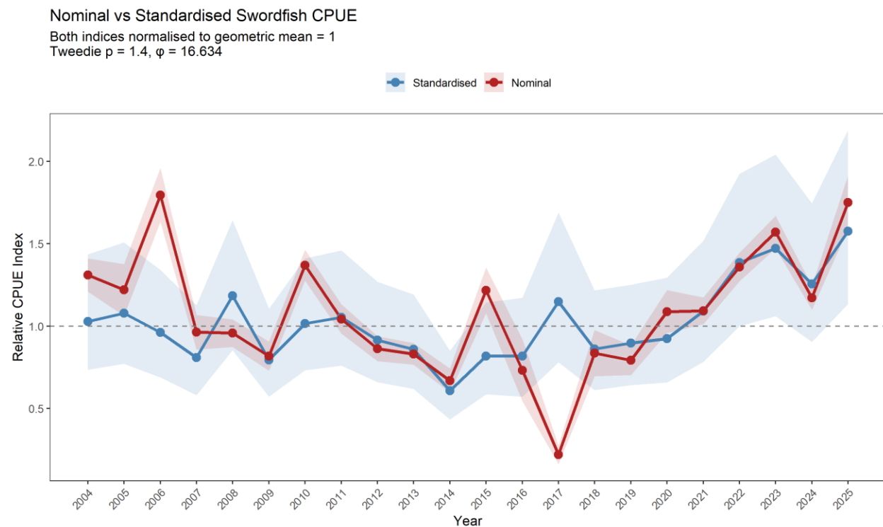
Figure 10. Standardised and nominal swordfish CPUE for the South African pelagic longline fishery for the period 2004 to 2025, normalised by the geometric mean. The 95% confidence intervals are denoted by shaded areas.
