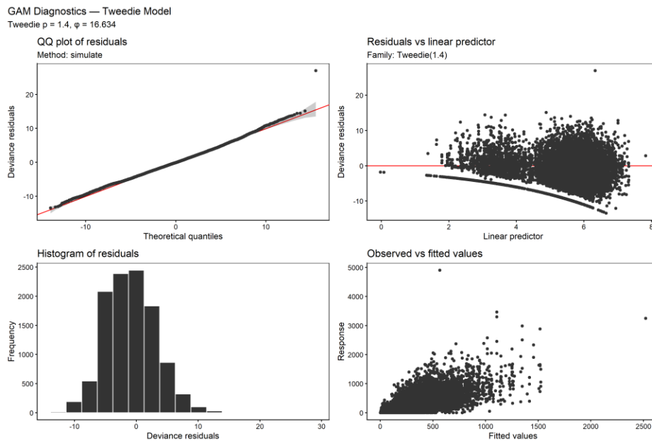
Figure 6. Diagnostic evaluation of the tweedie standardisation model.
