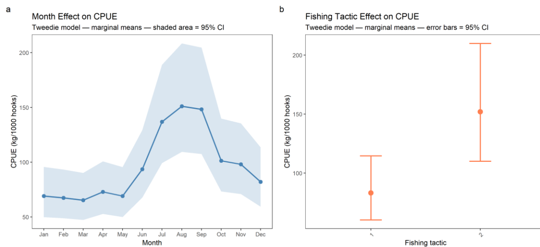
Figure 8. The influence of the fixed effects Month and Fishing Tactic on the CPUE of swordfish when modelled using the tweedie model applied to the South African longline data.
