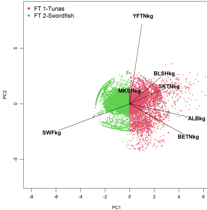
Figure 5. A graphical representation of the two clusters that characterise the different fishing tactics projected over the first two Principal Components (PCs). Fishing Tactic 1 (FT1): Cluster one (red) is predominantly tunas (yellowfin, bigeye, albacore) and shark (blue and shortfin mako) catch. Fishing Tactic 2 (FT2): Cluster two (green) is swordfish.
