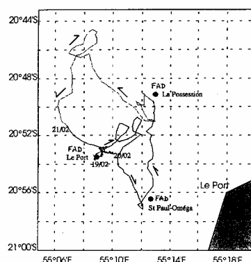
Figure 2. Tracking course of the YF1 (FL=110cm). Feb. 19, 1994, 11:00 am to Feb. 21, 6:30 am.
