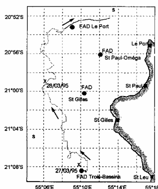
Figure 3. Tracking course of the YF5 (FL=104cm). March 27, 1995, 10:55 am to March 28, 7:33 am.
