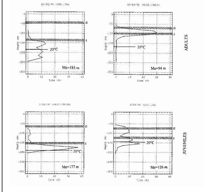
Figure 13. Relative time at depth for transit swimming at daytime.
