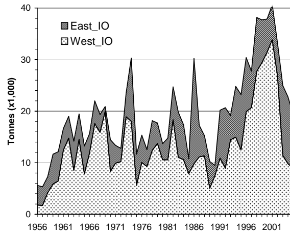
Figure 4: Catches of albacore in relation to the eastern and western areas of the Indian Ocean (1956-2005). Data as of October 2006
