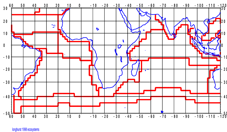
Figure 2. Ecological areas as proposed by Longhurst (1998)
