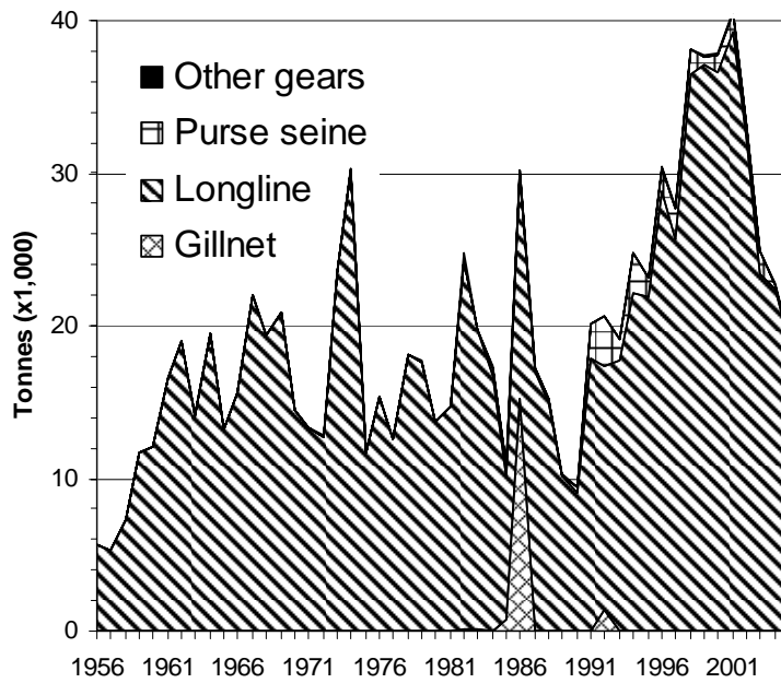
Figure 3. Albacore: Annual catches (thousand of metric tonnes) by gear from 1956 to 2005. Data as of October 2006
