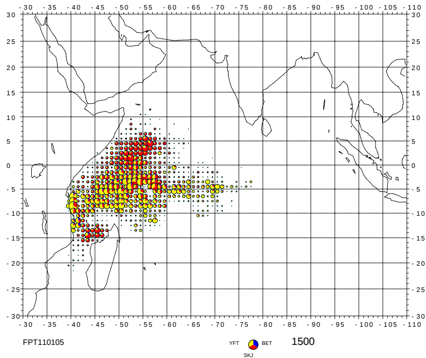
Figure 7a: Spatial distribution of the French fleet total catches in 2006 and for the average situation over the period 2001-2005
