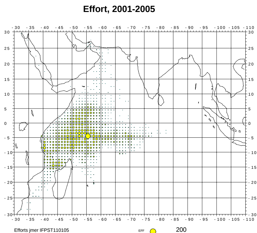
Figure 7b: Spatial distribution of the French fleet total effort (fishing days) in 2006 and for the average situation over the period 2001-2005
