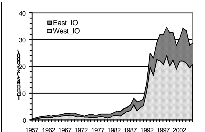
Figure 2. Trends of the swordfish catches in the western and the eastern area of the Indian Ocean from 1956 – 2006.
