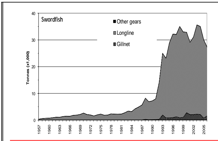
Figure 1. Catches of Swordfish per gear and year recorded in the IOTC Database (1957-2006).
