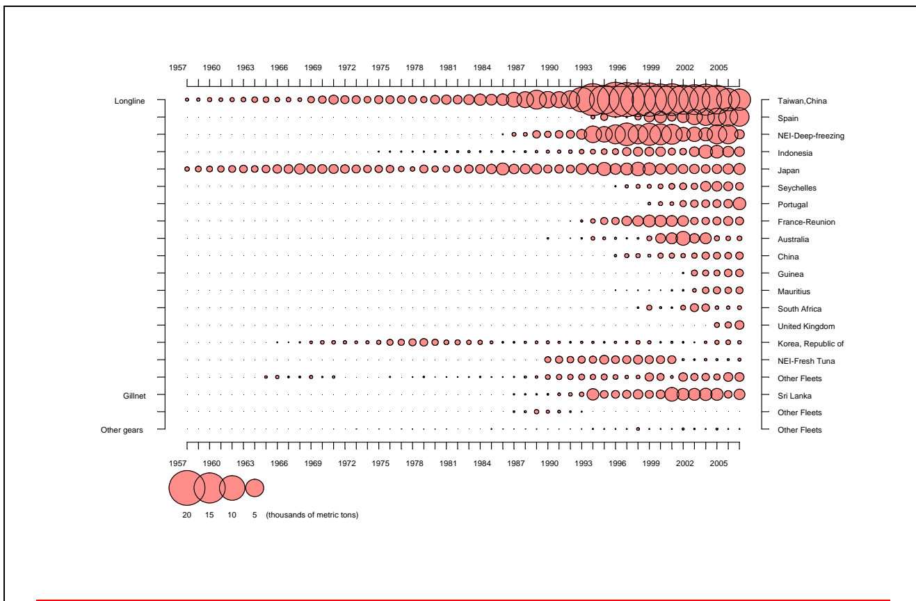
Figure 3. Catches of swordfish in the Indian Ocean for the period 1957-2006, in thousands of metric tons by gear and country/fleet. Data as of October July 2007
