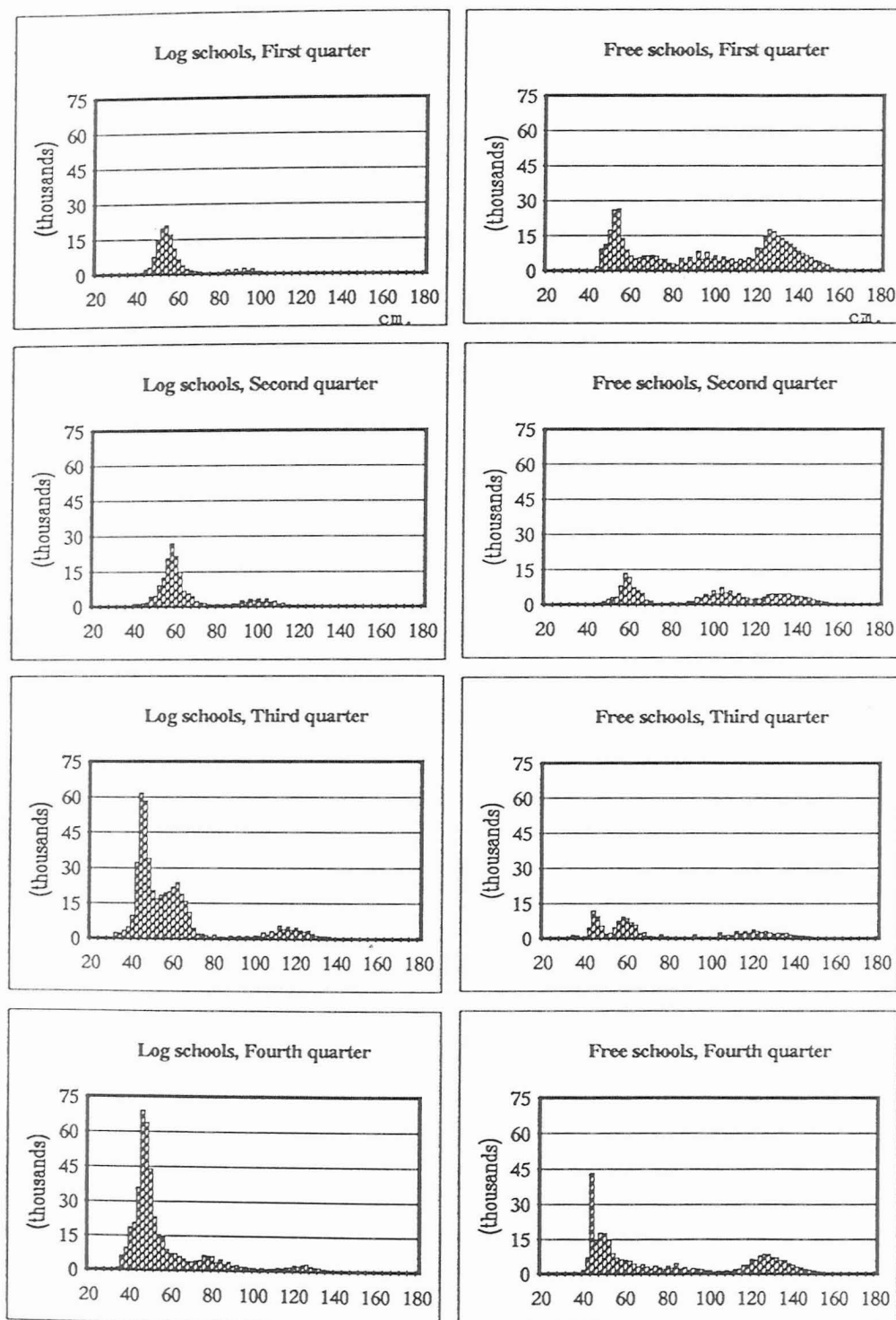
Figure 10: Seasonal variations by quarter of log associated (left) and free swimming (right) schools of the French-Ivory Coast purse-seine mean catch size composition, 1982-90.
