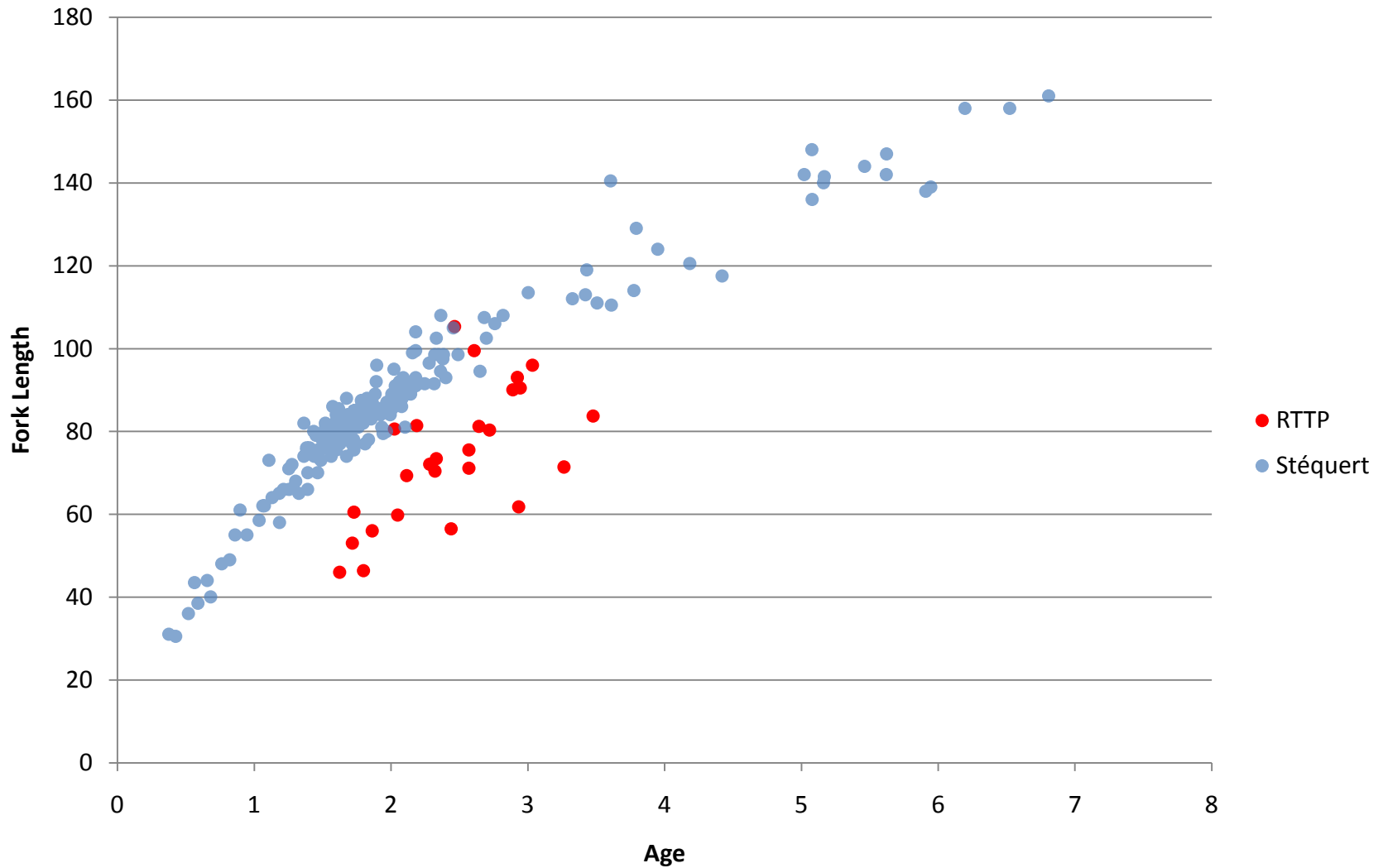
Figure 3. Comparison of the age calculated from the new data (n=26) with the Stéquent data (n=164).
